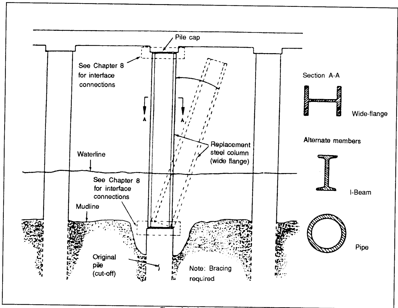
Figure A-8. Steel Columns
