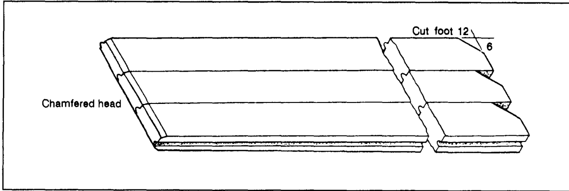
Figure 8-4. Planking
