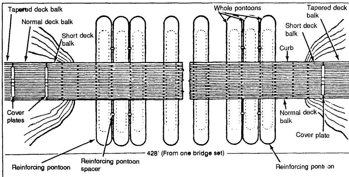
Figure 10-3. Causeway Using Reinforced Construction
