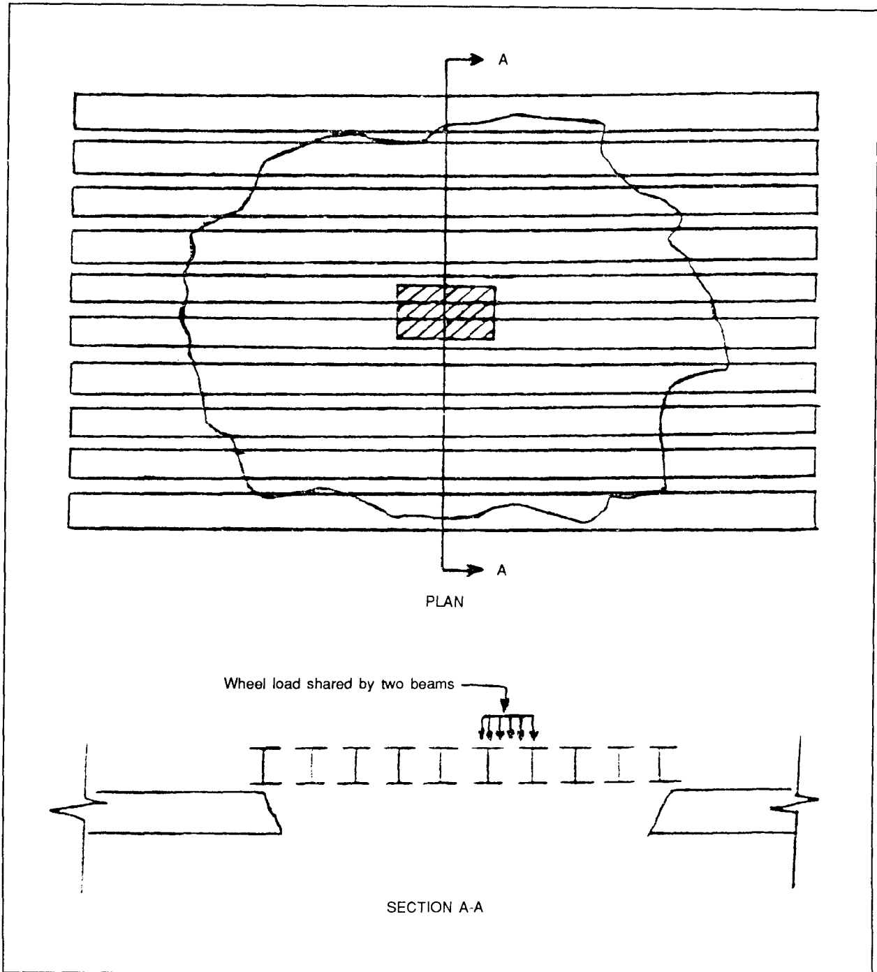
Figure A-40. Steel Beam Mat Concept Repair
