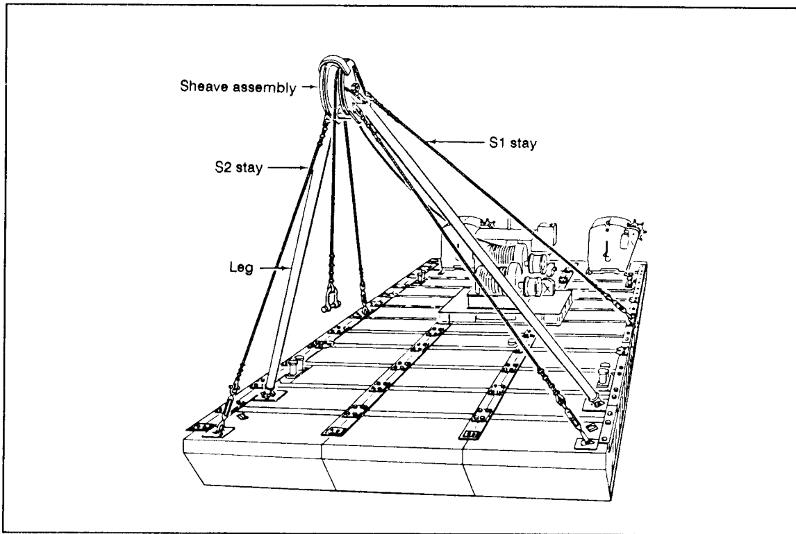
Figure 10-13. Assembled 3 by 14 Warping Tug with A-Frame
