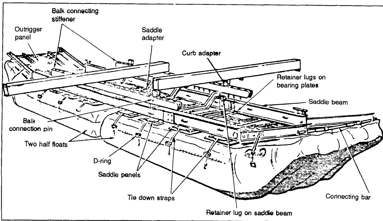
Figure 10-1. M4T6 Float Section
