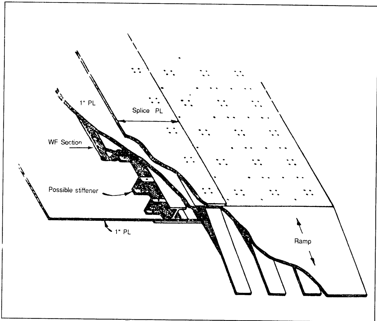
Figure A-30. Isometric View of Type A Module
