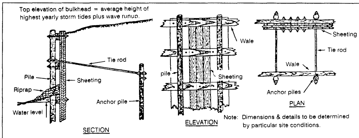
Figure 5-3. Timber Bulkhead
