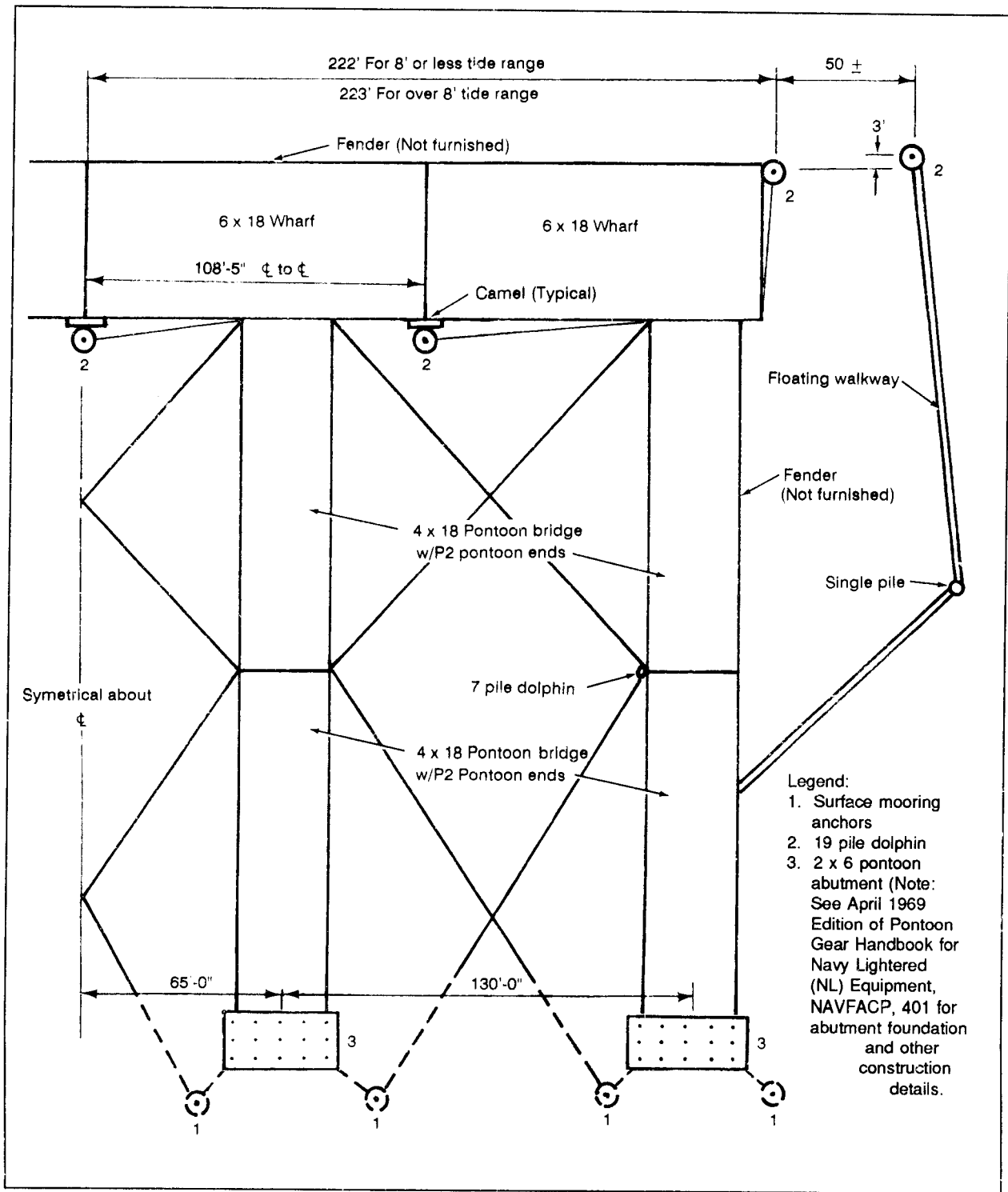
Figure 10-17. Causeway Arrangement 2 (with Pontoon Wharf)
