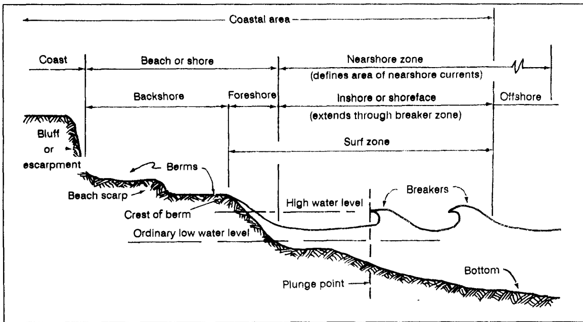
Figure 5-1. Beach Profile
