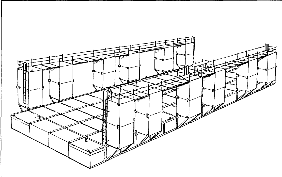
Figure 10-14. 4 by 15 Pontoon Drydock
