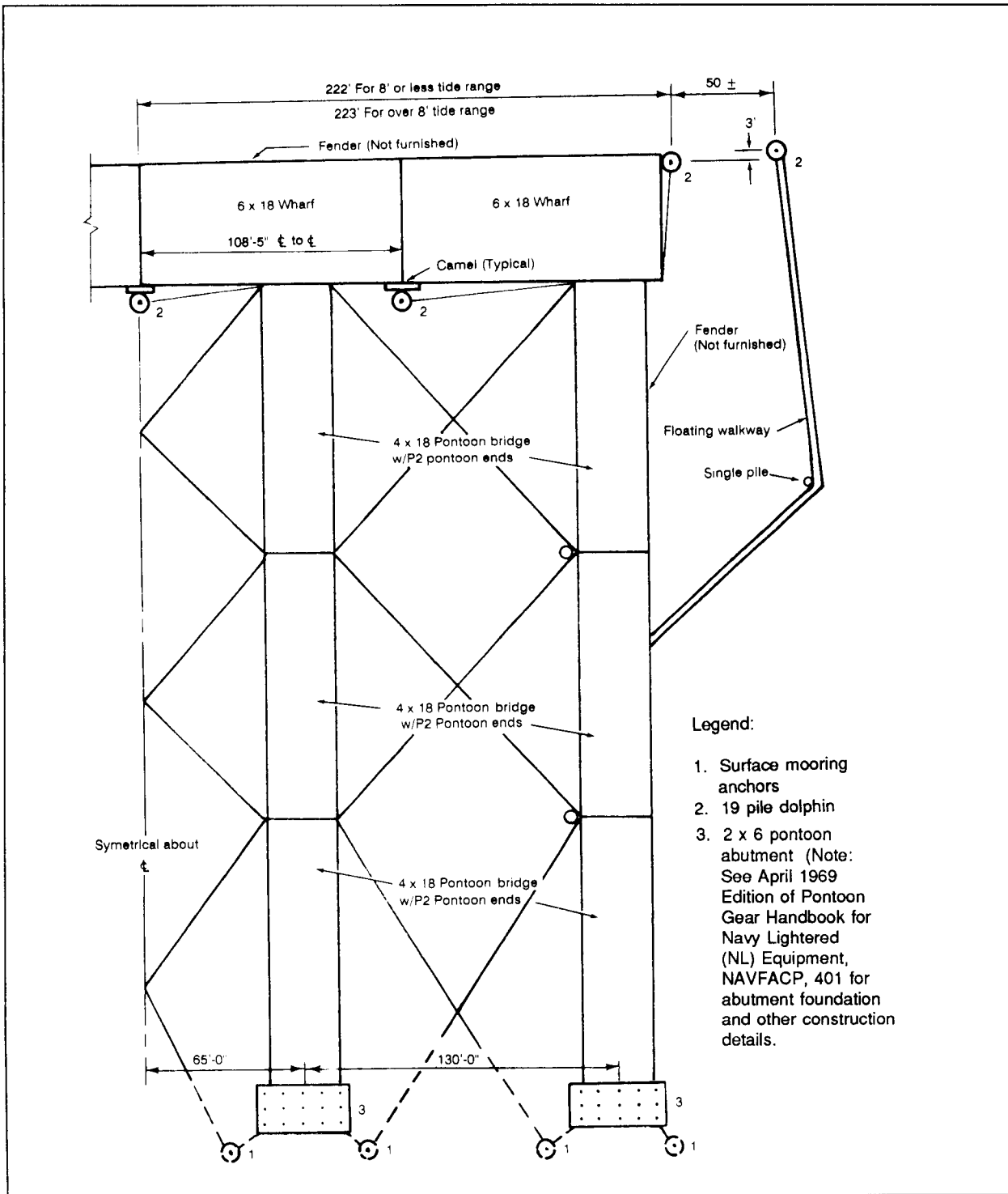
Figure 10-18. Causeway Arrangement 3 (with Pontoon Wharf)
