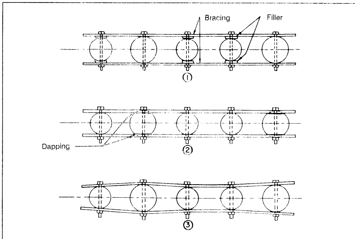
Figure 8-19. Flexible Braces
