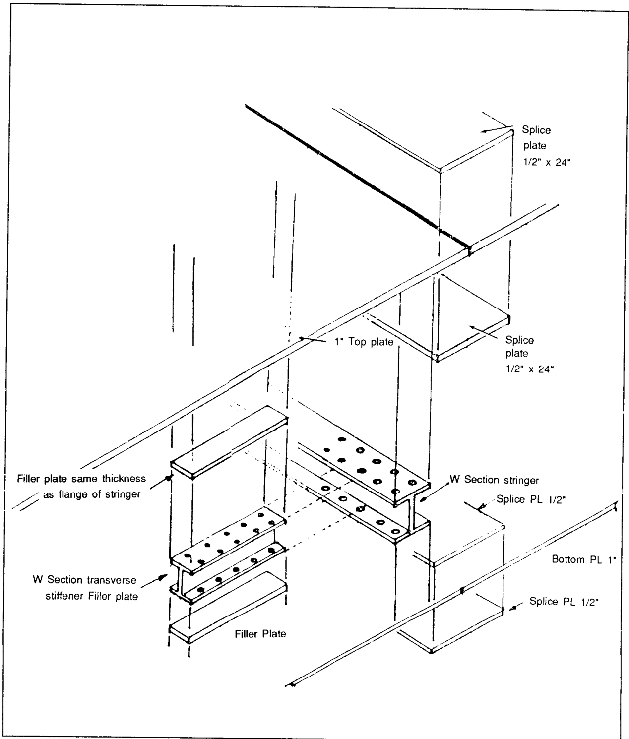
Figure A-32. Exploded Isometric View (Type A Repair Module)
