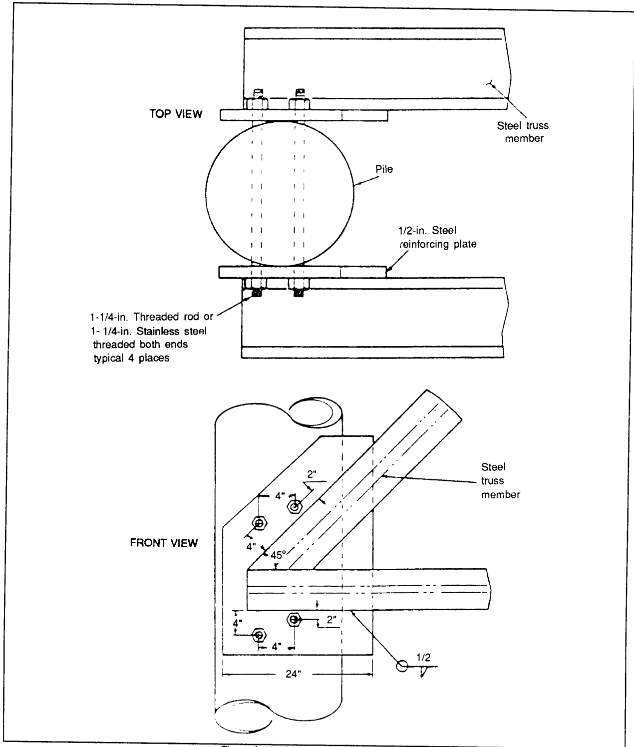
Figure A-16. Steel Truss Pile Connection
