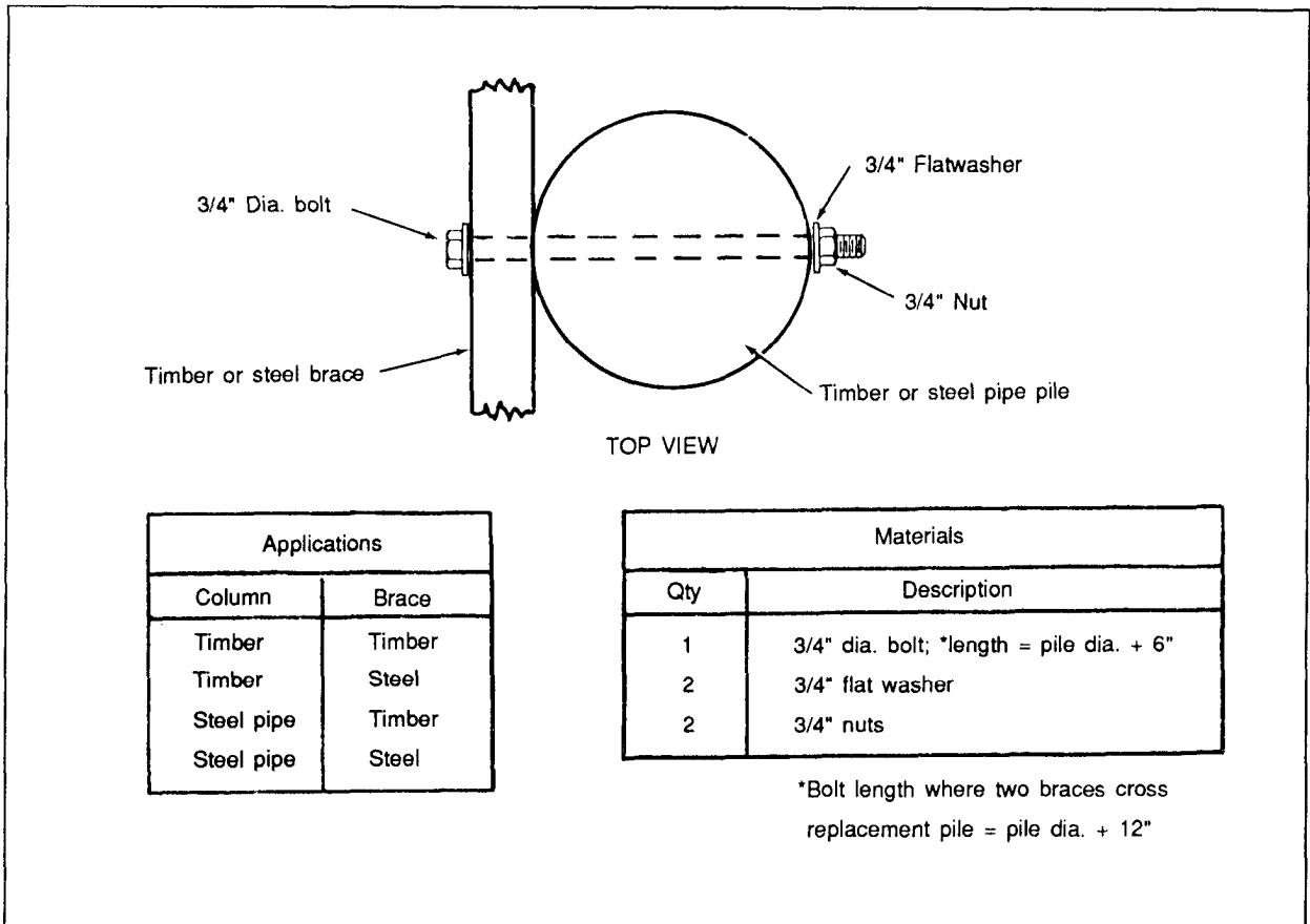
Figure A-18. Brace Connected to Timber or Steel Pipe Pile (Bracing Method 1)
