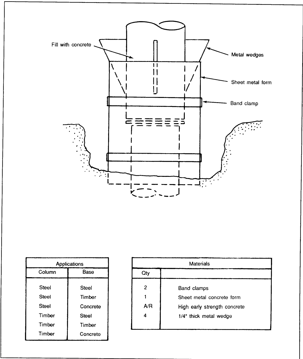
Figure A-28. Joining Piles at the Ocean Floor with Concrete, Column to Base Connections (Connecting Method 7)
