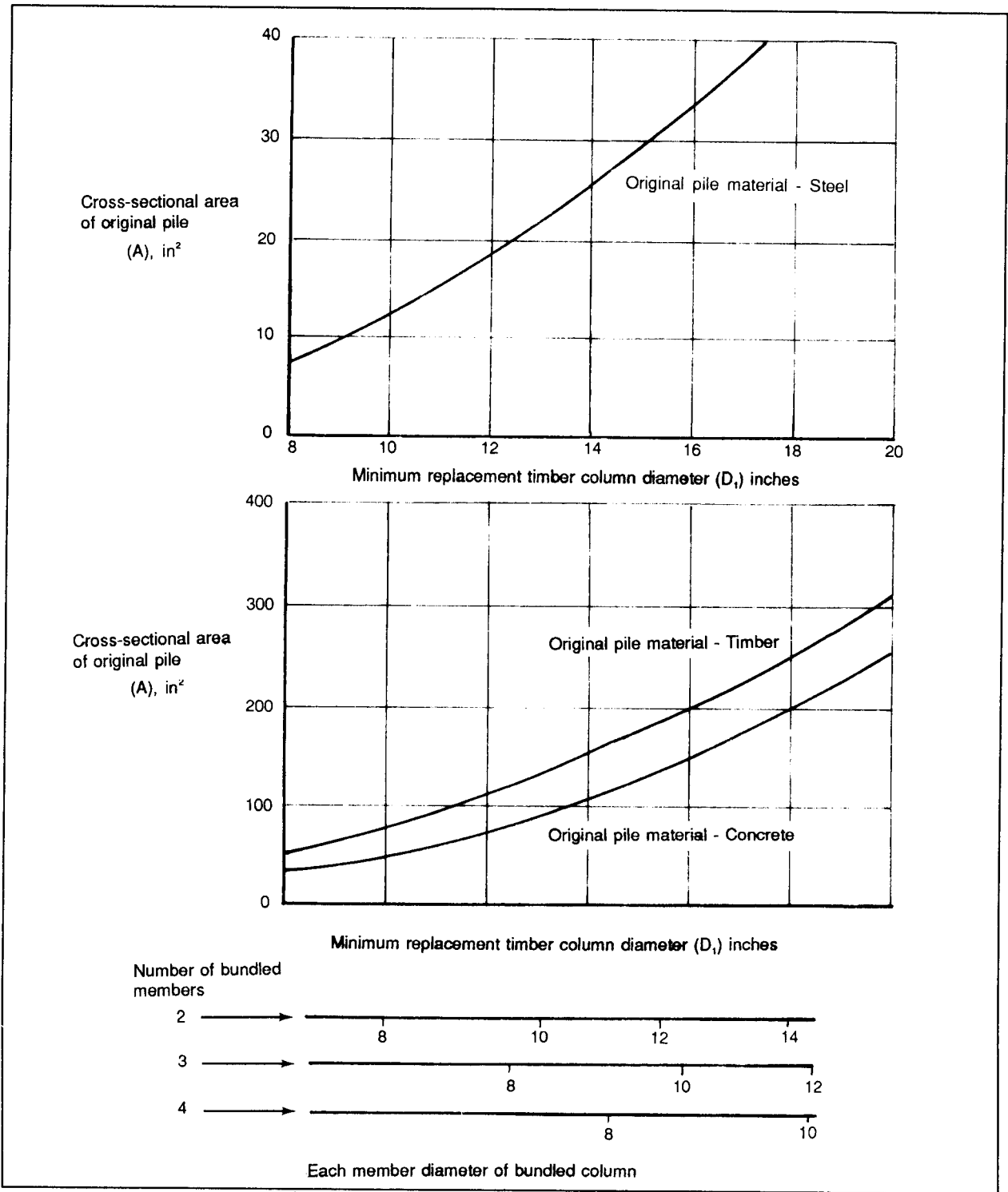
Figure A-4. Replacement Timber Diameter Determination
