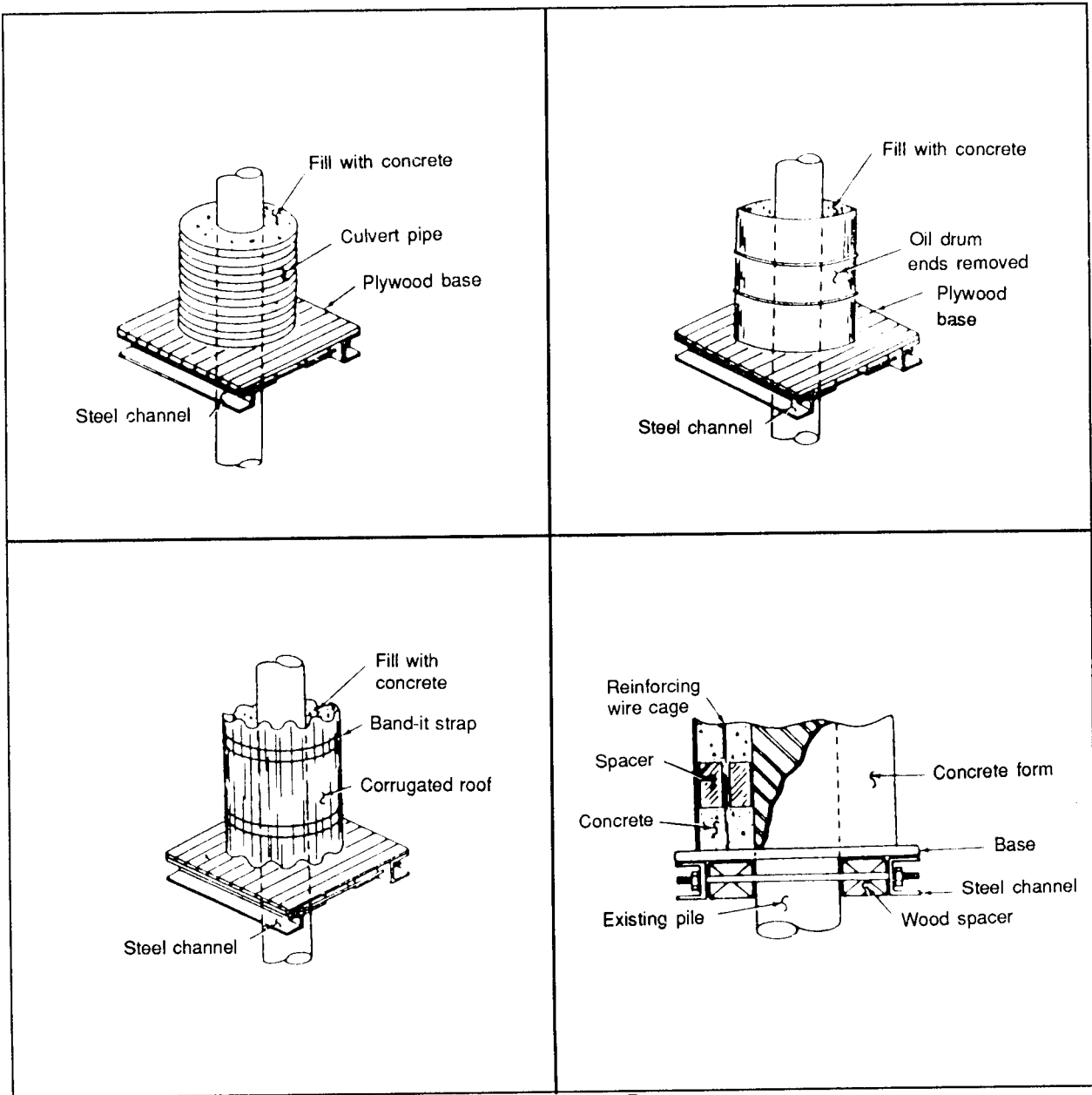
Figure A-11. Alternate Forms
