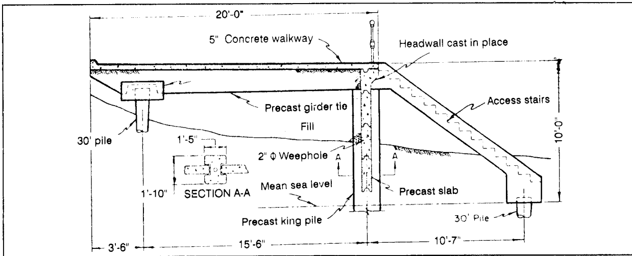
Figure 5-4. Concrete Bulkhead
