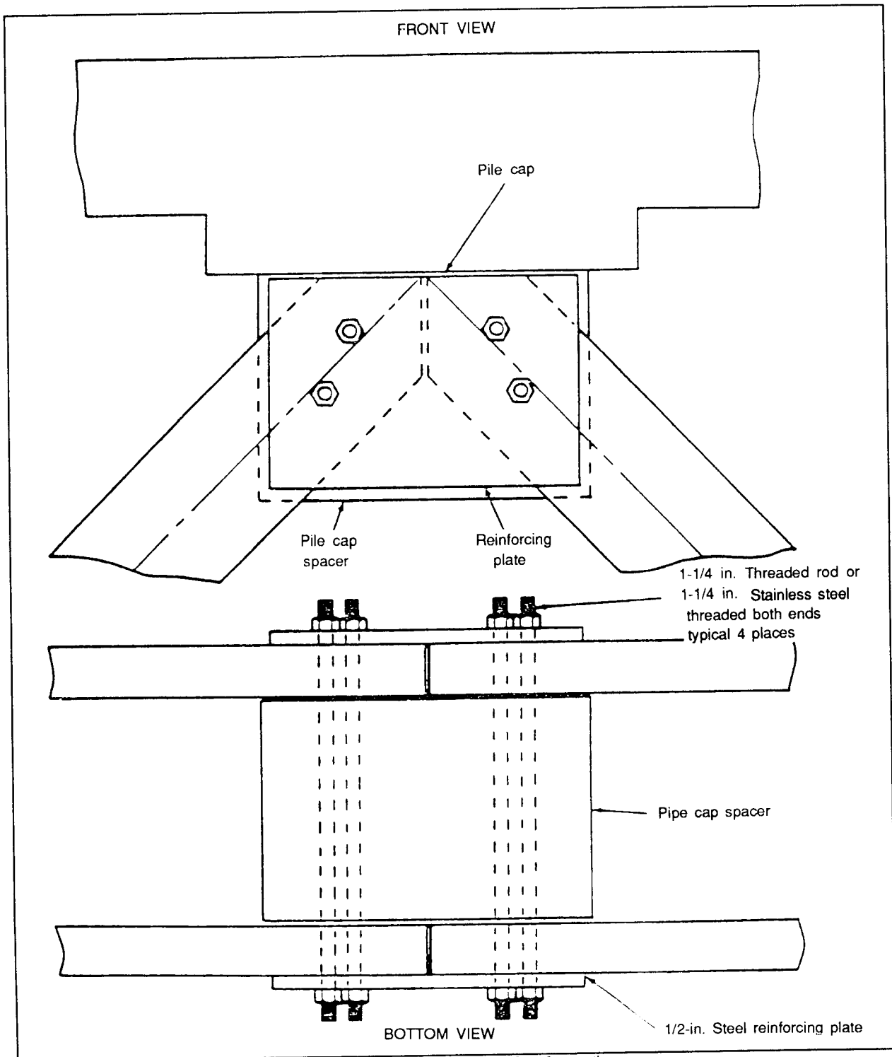
Figure A-13. Timber Truss Pile Cap Connection
