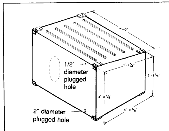
Figure 10-6. P3 Pontoon
