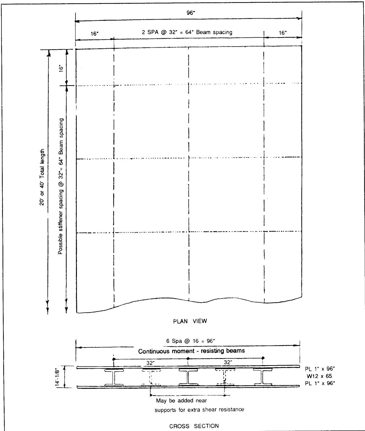
Figure A-31. Plan and Cross Section (Type A Repair Module)
