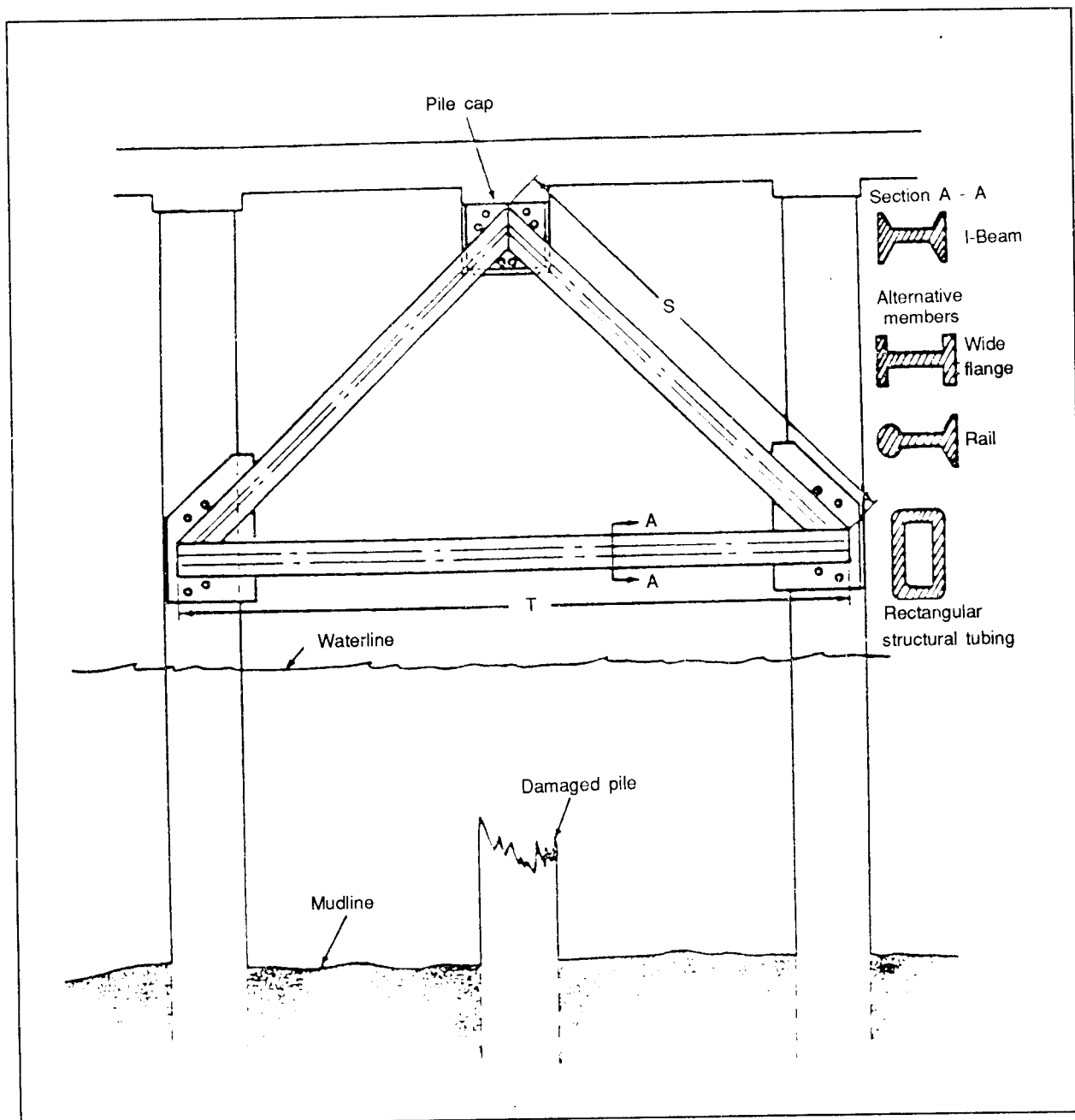
Figure A-15. Steel Truss
