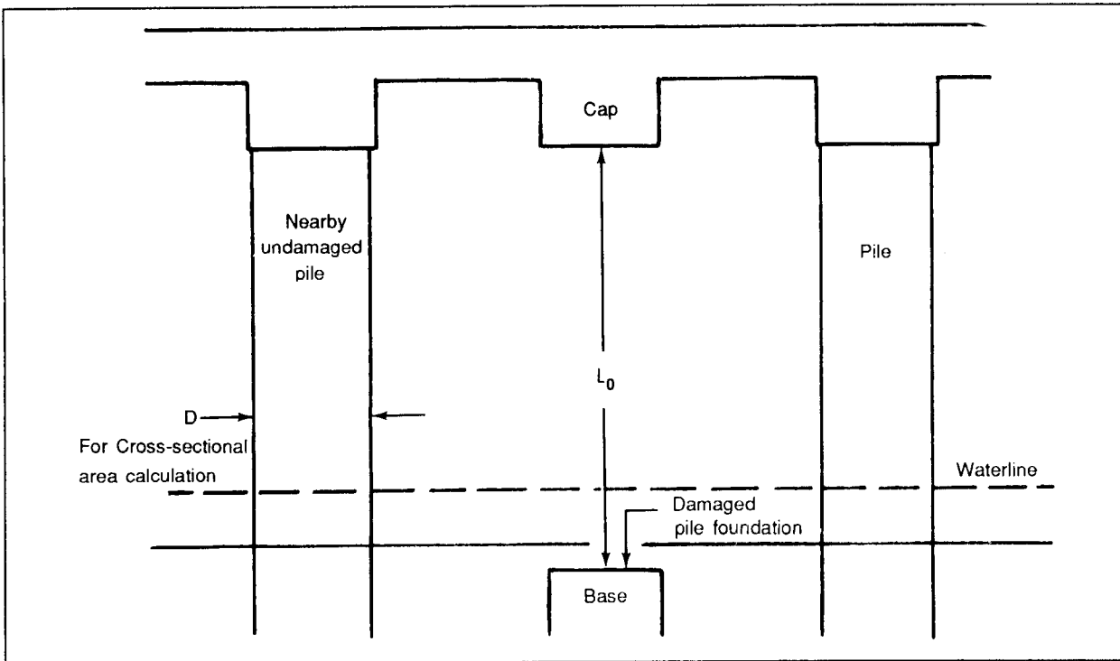
Figure A-2. Structural Elements of Pier or Wharf with Damaged Pile
