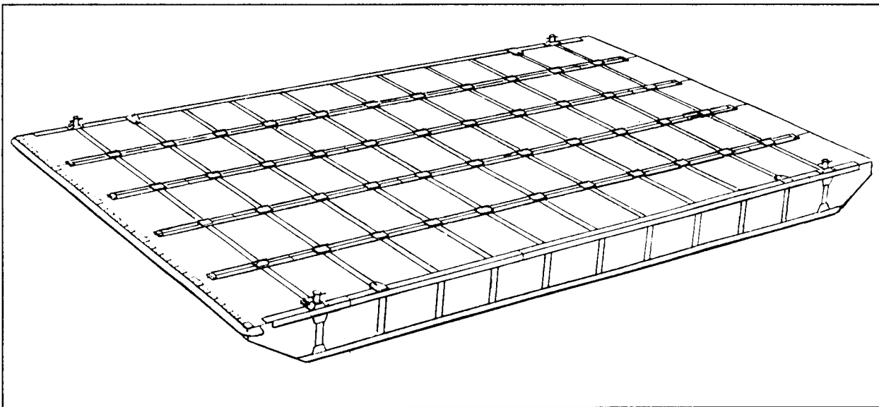
Figure 10-10. 5 by 12 Pontoon Barge
