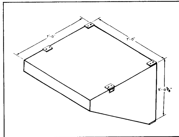
Figure 10-5. P2 Pontoon
