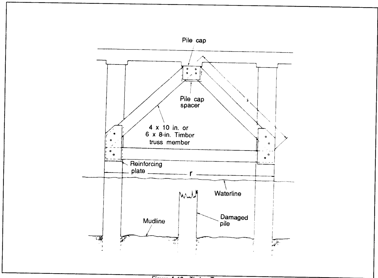
Figure A-12. Timber Truss
