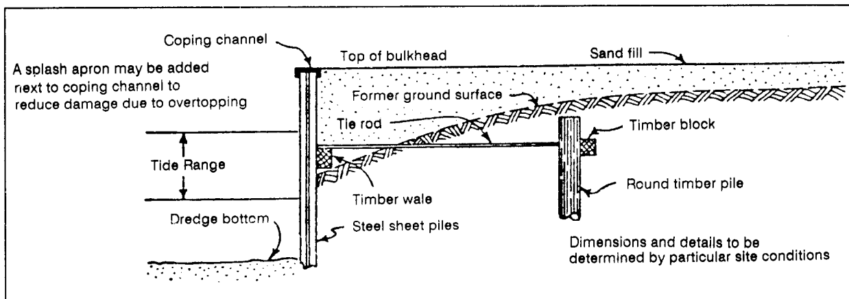
Figure 5-5. Steel Bulkhead
