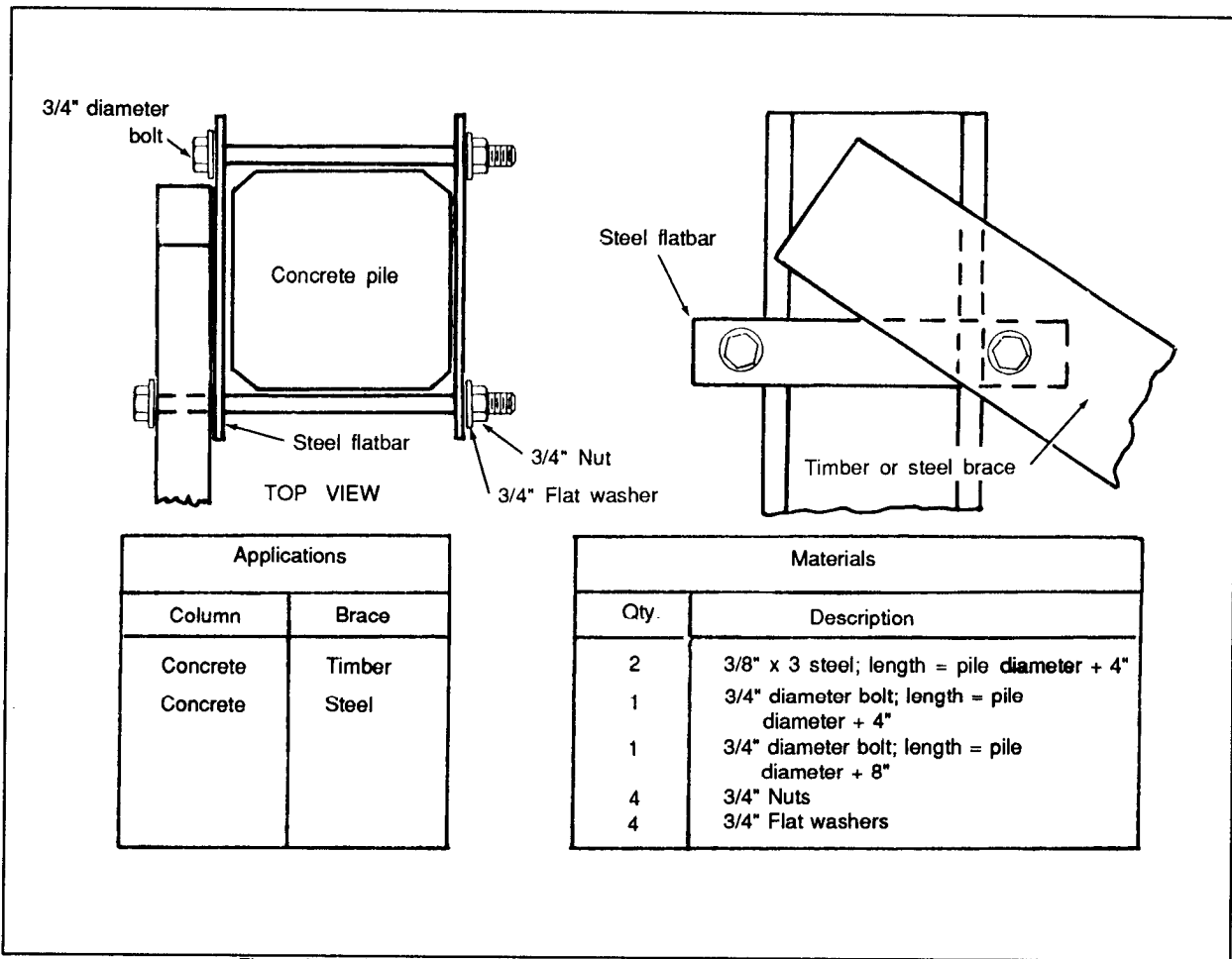
Figure A-20. Brace Connected to Concrete Pile (External Bracket-Bracing Method 3)
