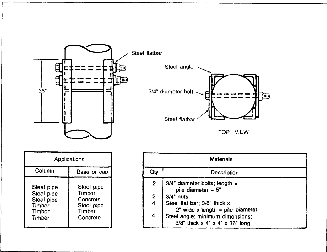
Figure A-24. Joining Like-Diameter Piles, Column to Base or Cap Connections (Connecting Method 3)
