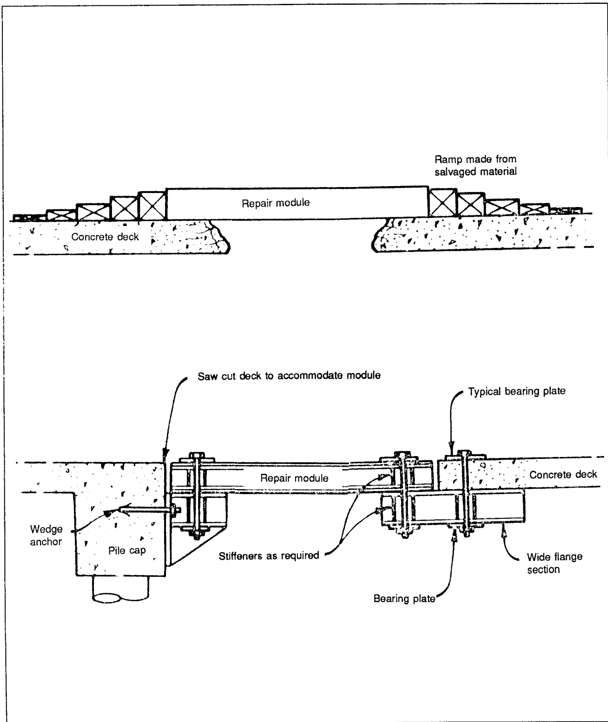
Figure A-33. Alternate Installation Methods for Repair Modules (Type A or B)
