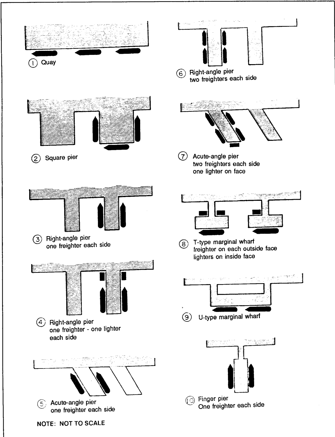
Figure 3-1. Wharf Layout
