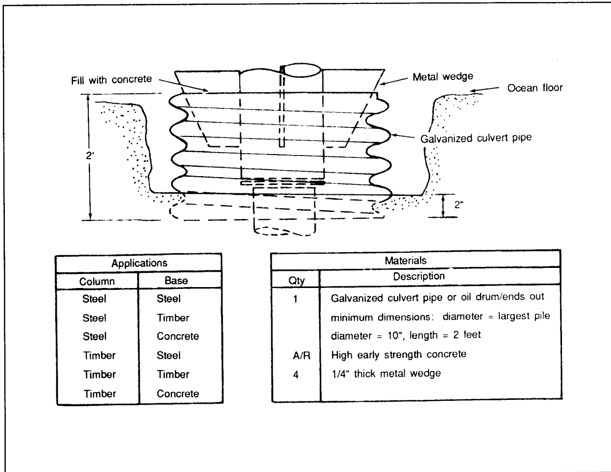
Figure A-27. Joining Piles at the Ocean Floor with Concrete, Column to Base Connections (Connecting Method 6)
