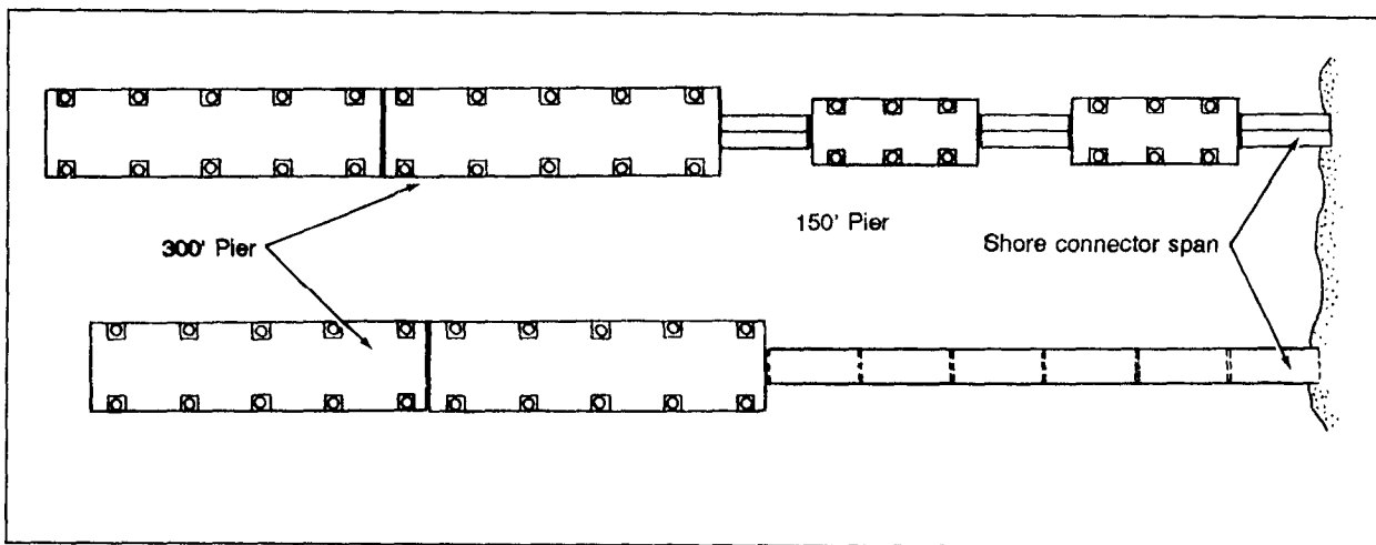
Figure 11-4. Finger Piers
