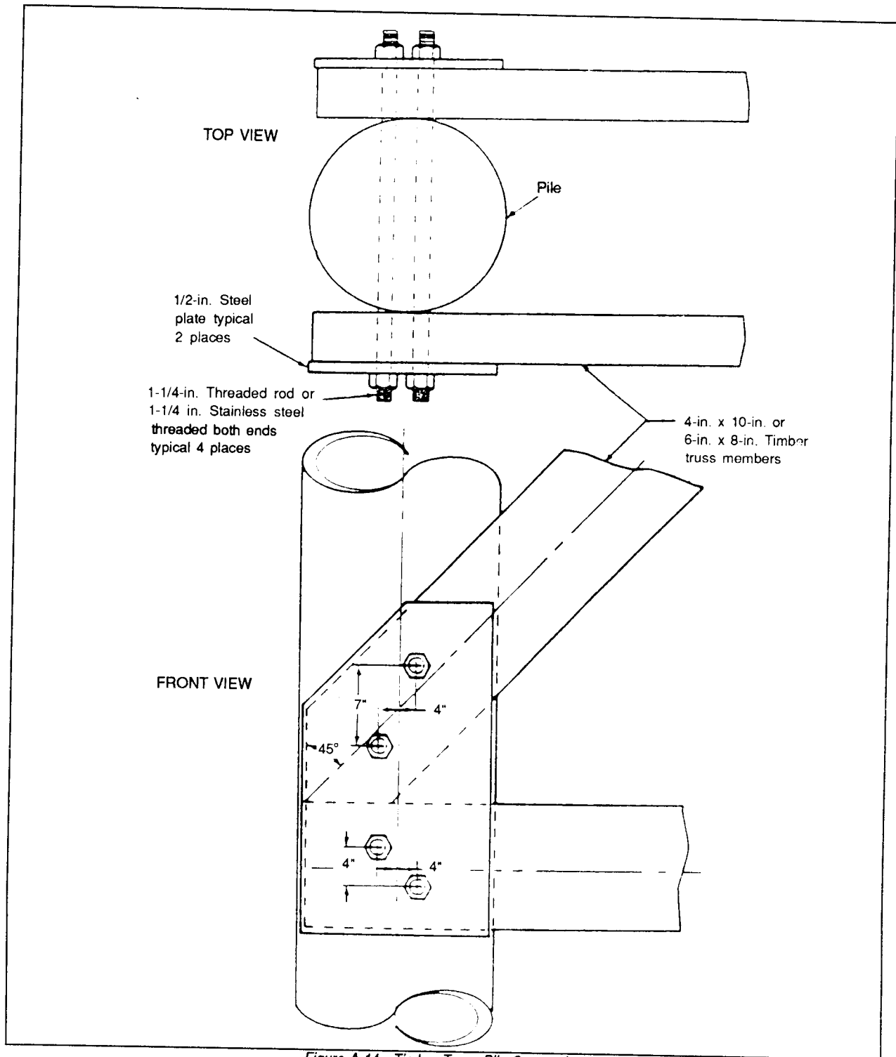
Figure A-14. Timber Truss Pile Connection
