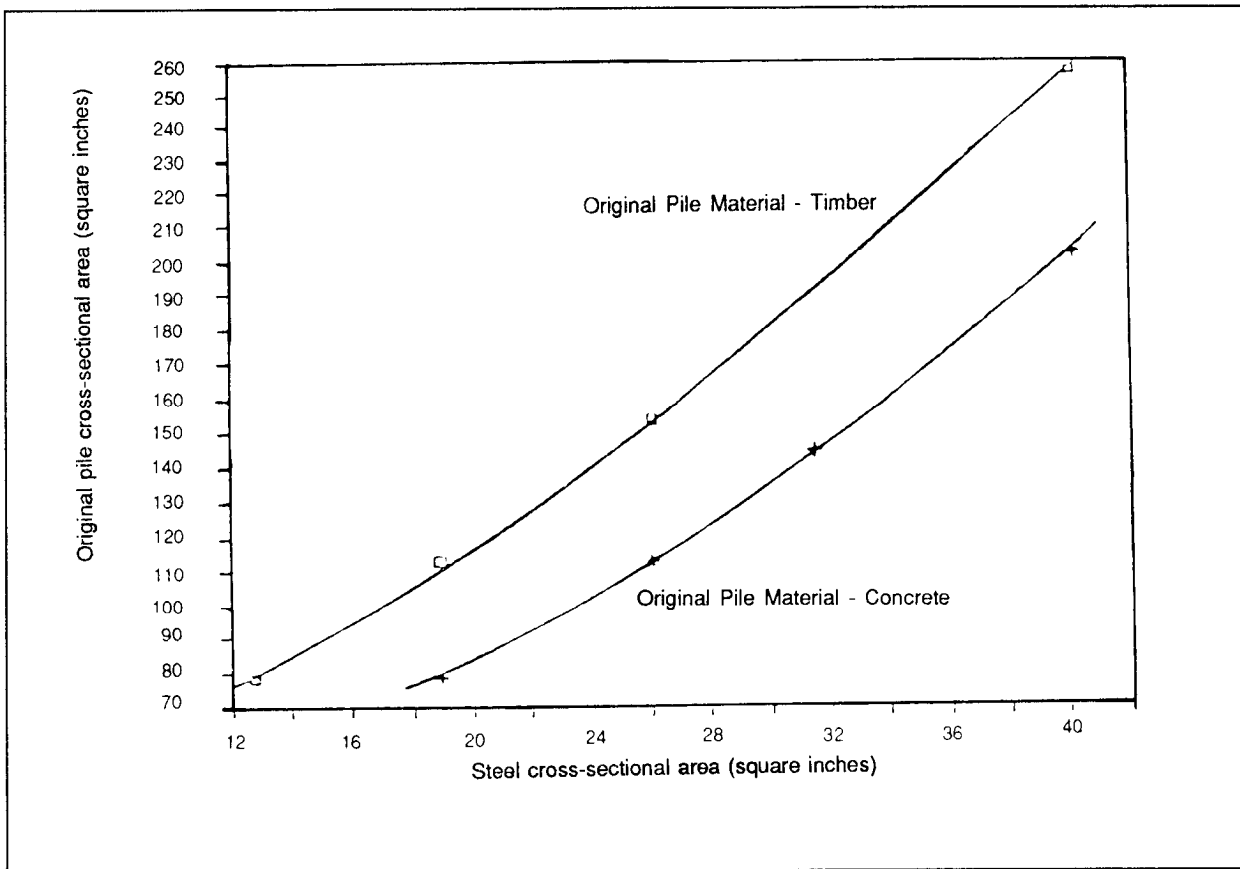
Figure A-5. Equivalent Steel Cross-Sectional Area
