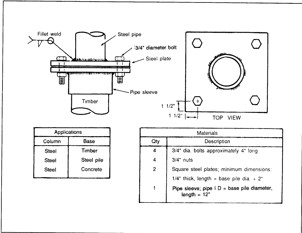
Figure A-26. Joining Steel Column to Base Pile, Column to Base Connections (Connecting Method 5)
