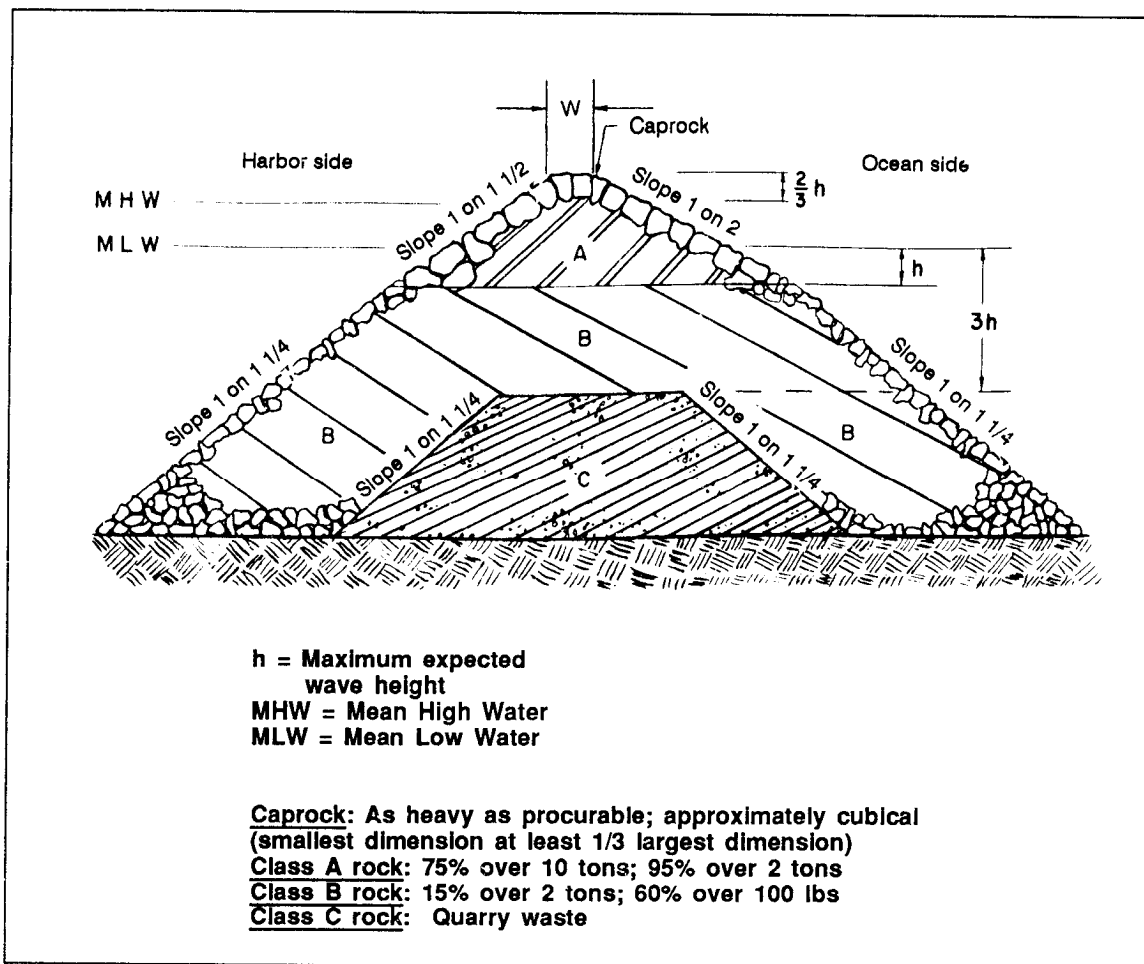
Figure 5-2. Rubble-Mound Breakwater
