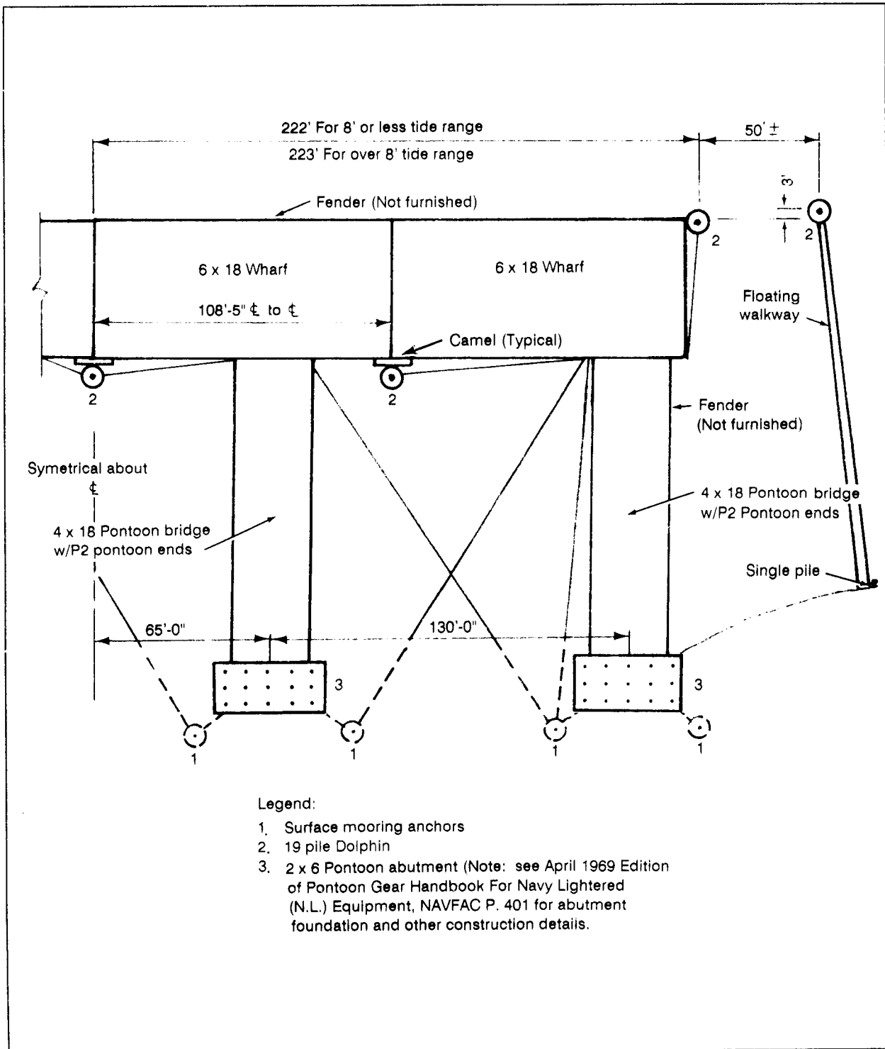
Figure 10-16. Causeway Arrangement 1 (with Pontoon Wharf)
