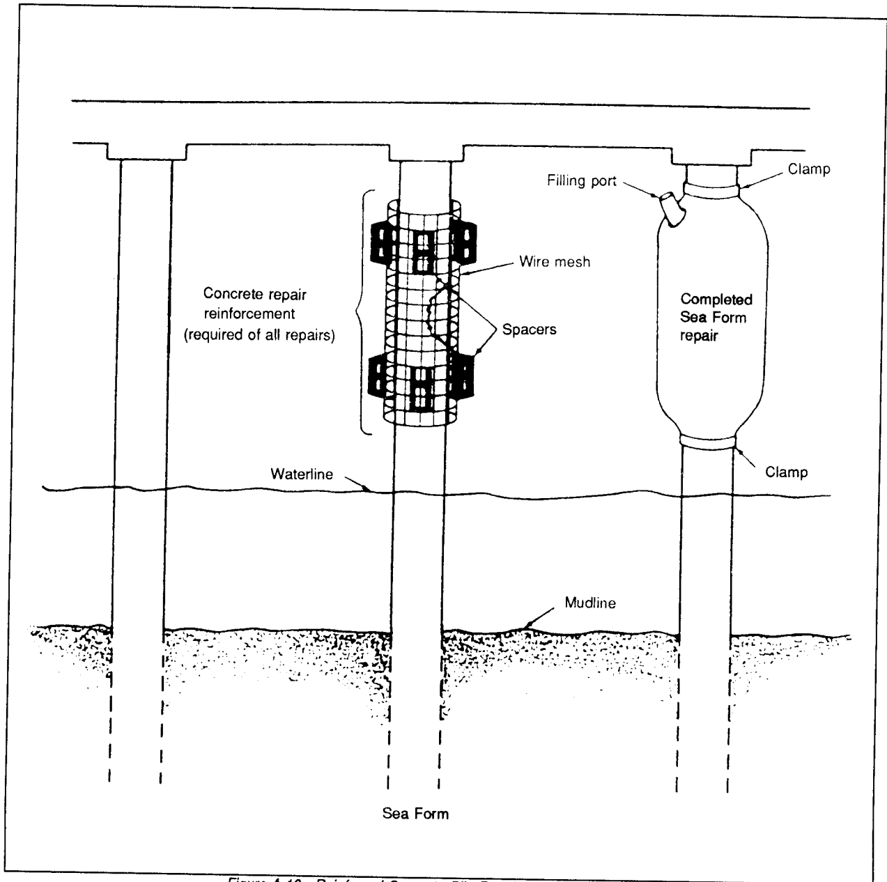
Figure A-10. Reinforced Concrete Pile Repairs Using "Sea Forms"
