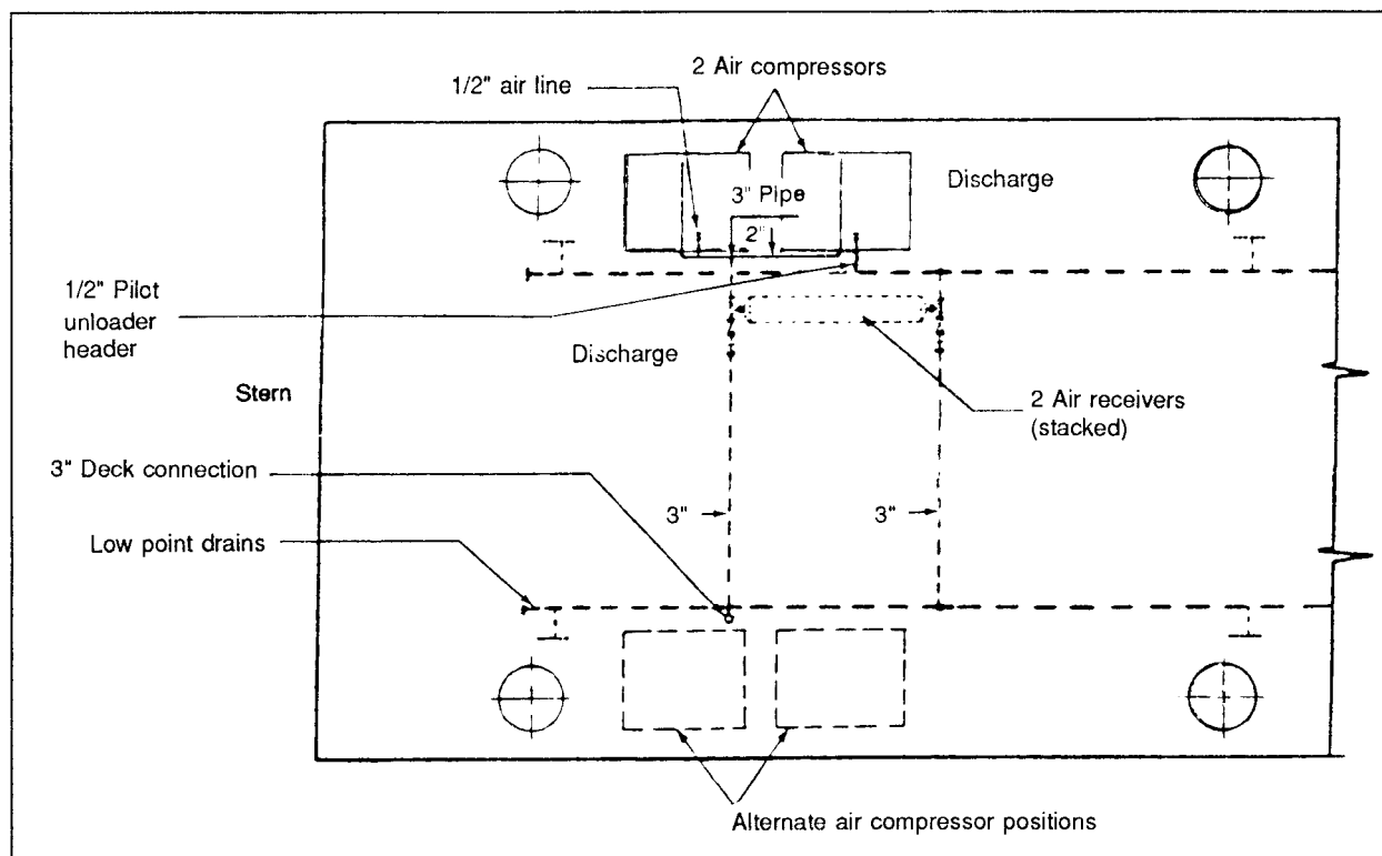
Figure 11-3. Compressor Positions
