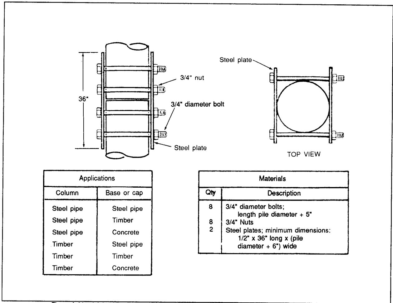
Figure A-22. Joining Like-Diameter Piles, Column to Base or Cap Connections (Connecting Method 1)
