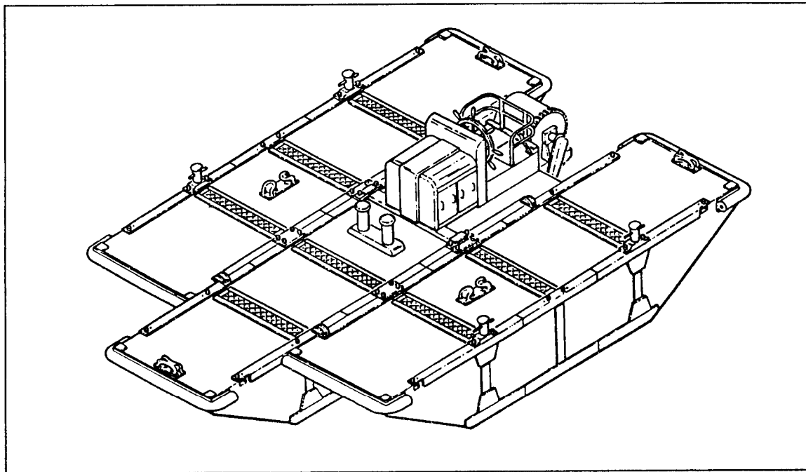
Figure 10-12. 3 by 4 Pontoon Tug
