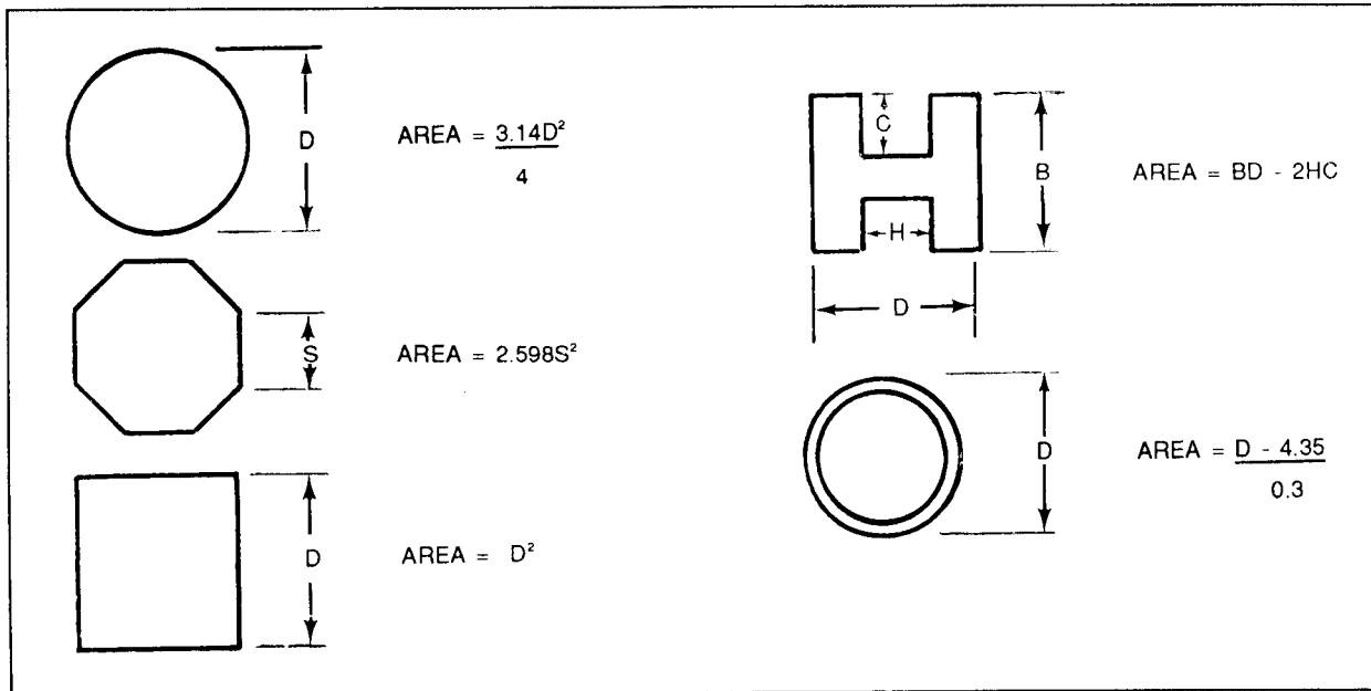
Figure A-3. Cross-Sectional Area Formulas for Adjacent Pile
