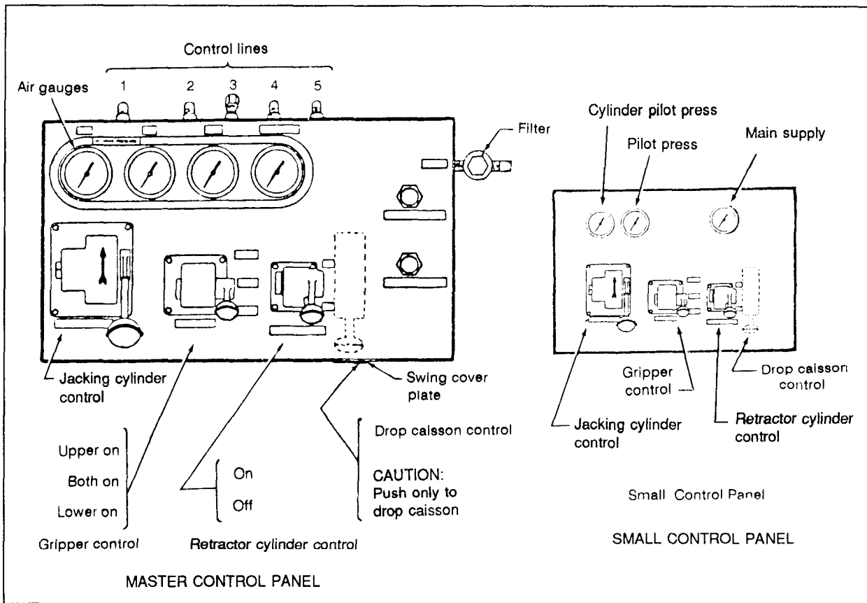
Figure 11-1. Control Panels
