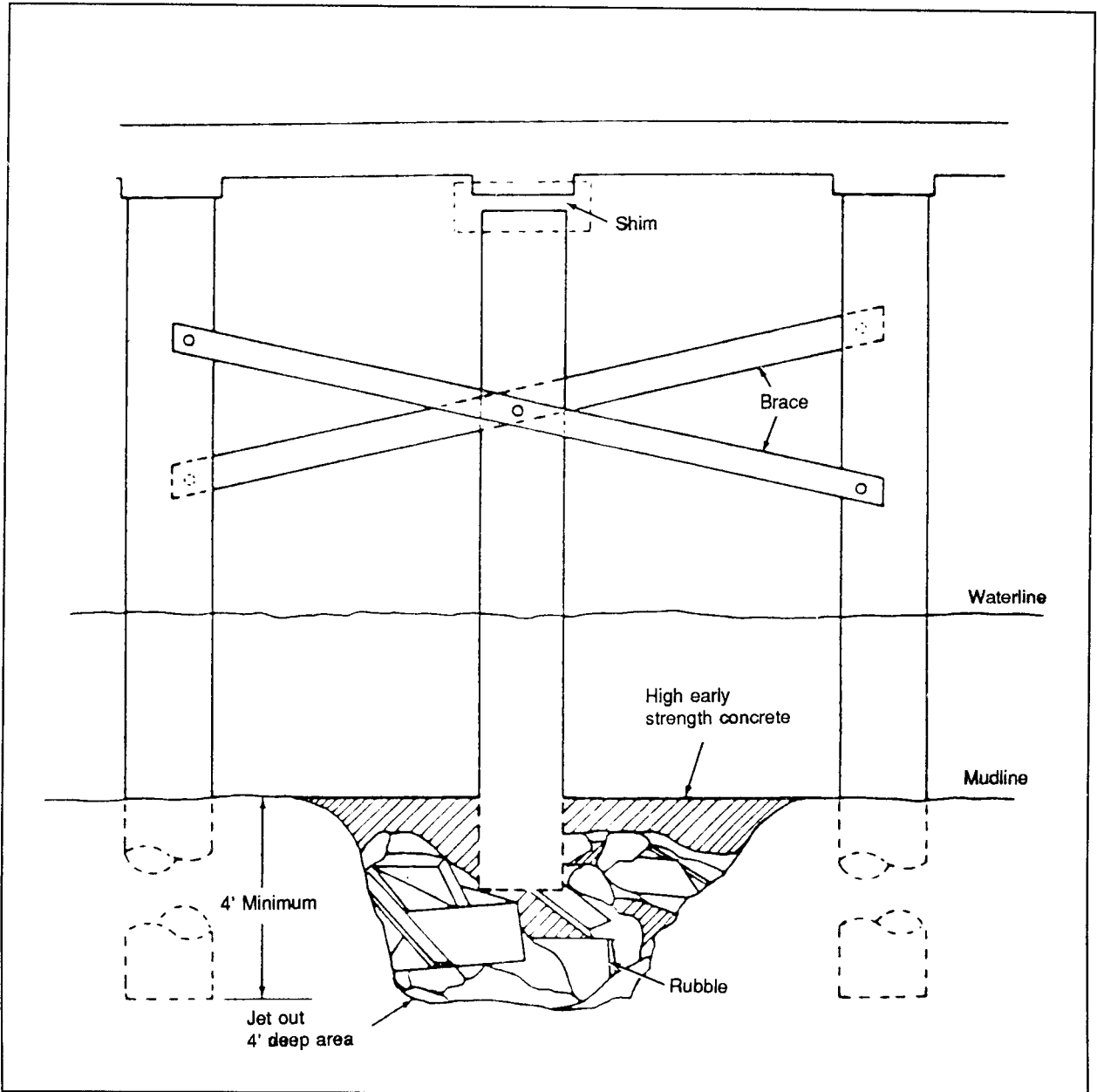
Figure A-1. Rubble Foundation
