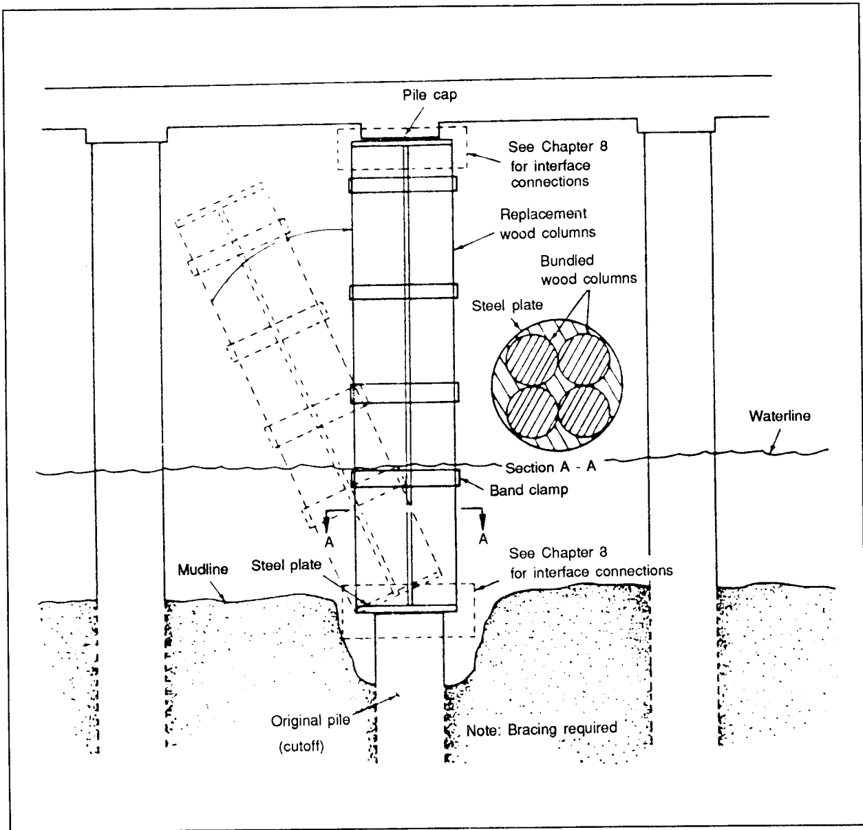
Figure A-7. Bundled Wood Columns
