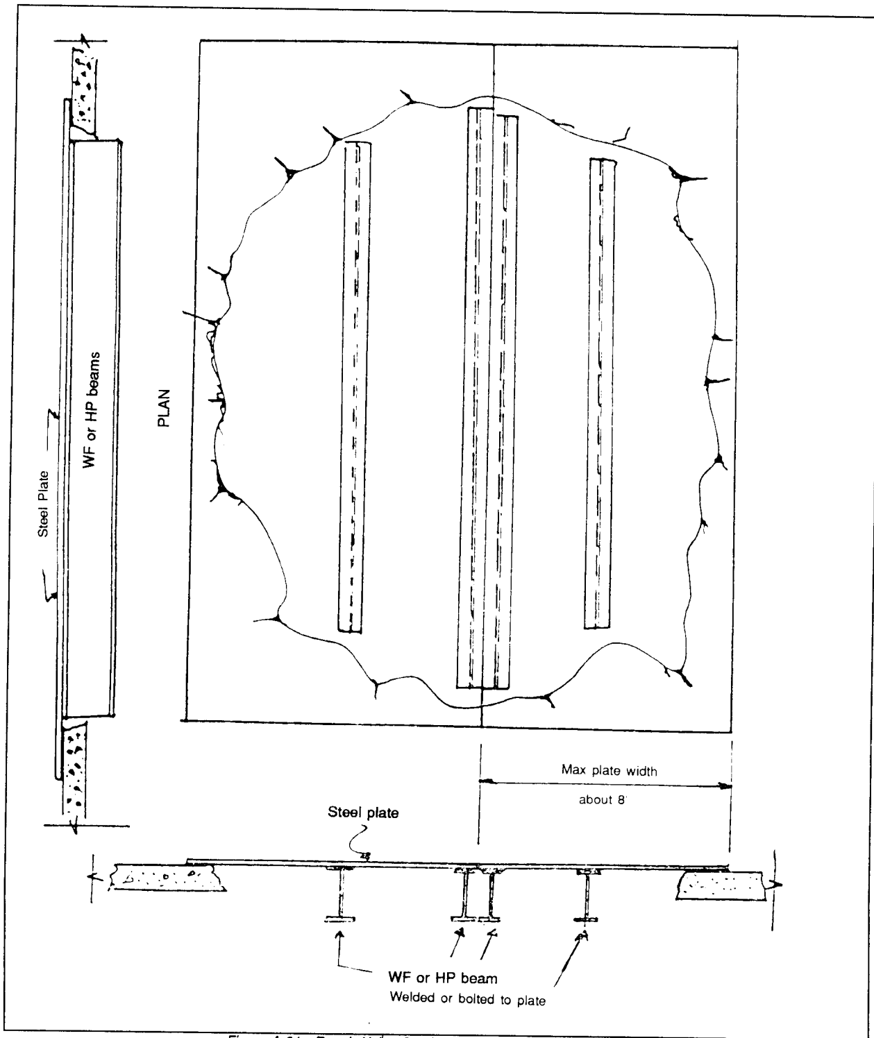
Figure A-34. Repair Using Steel Plate Reinforced by Steel Beams
