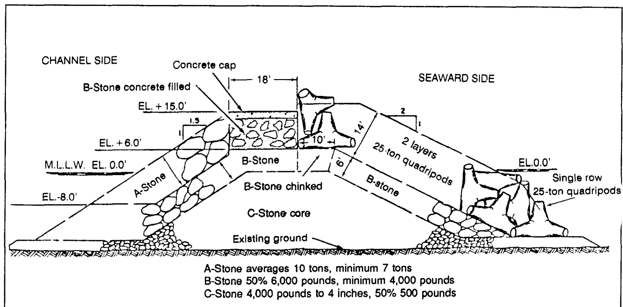
Figure 5-11. Quadripod Armor Units in Jetty Construction
