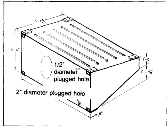
Figure 10-7. P4 Pontoon
