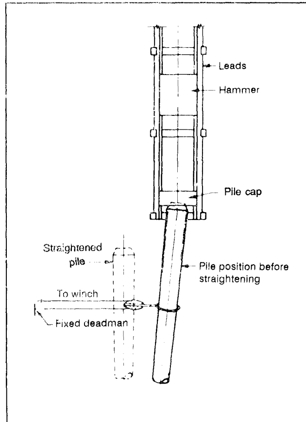
Figure 8-15. Straightening a Pile Using a Block and Tackle
