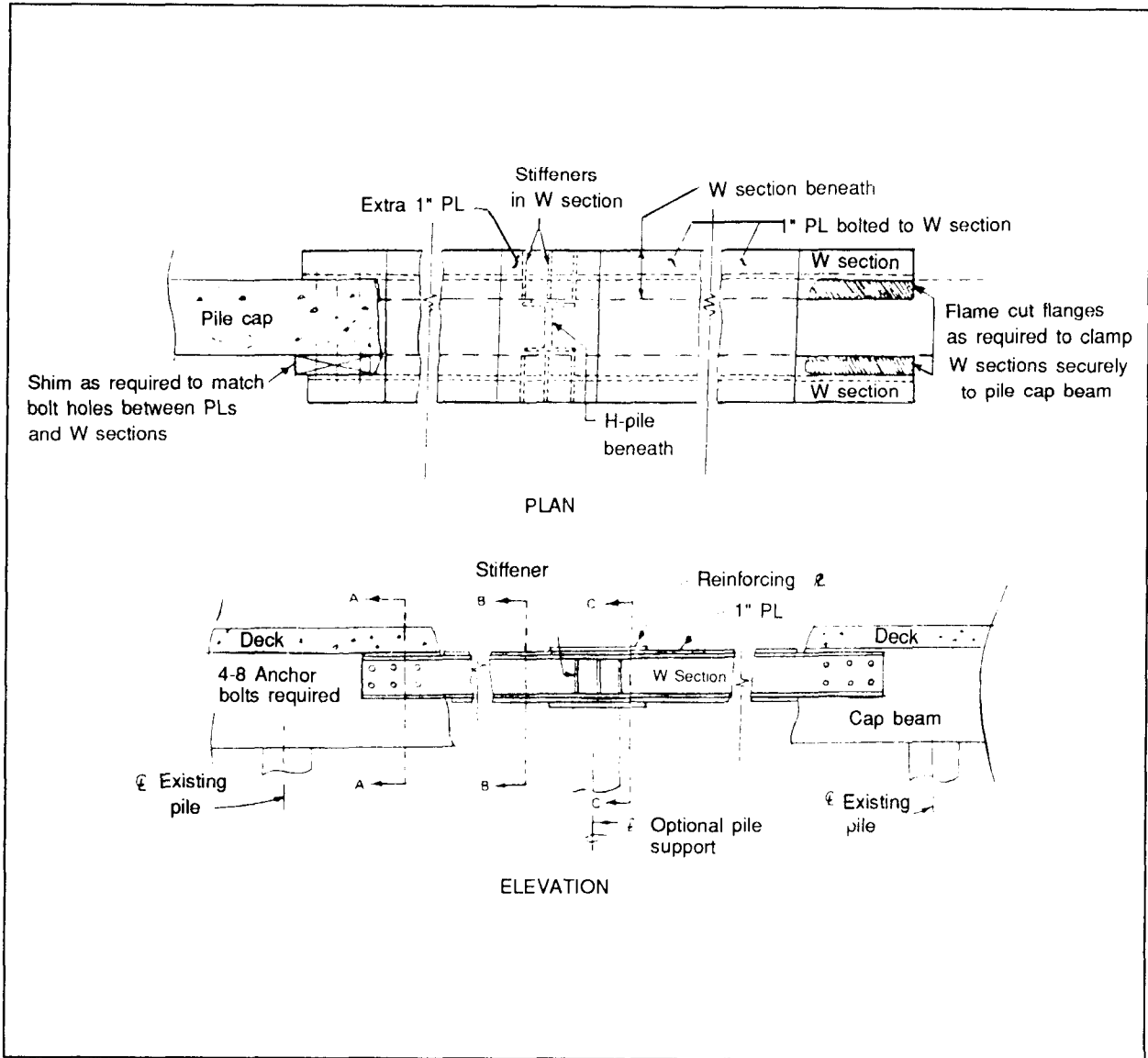
Figure A-36. Plan and Elevation Views of an Expedient Pile Cap
