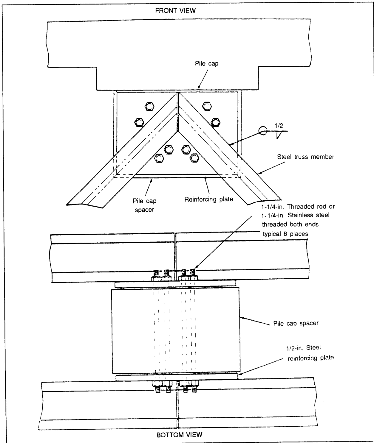
Figure A-17. Steel Truss Pile Cap Connection
