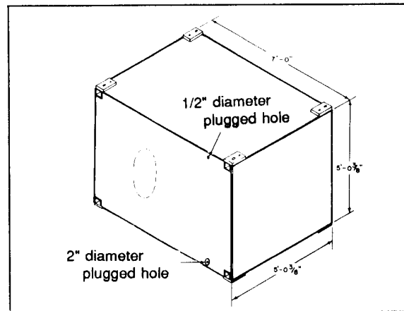
Figure 10-4. P1 Pontoon
