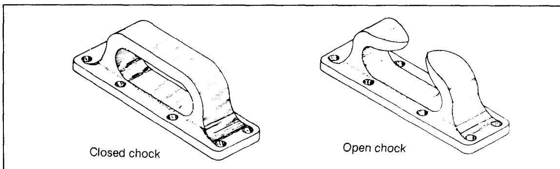
Figure 9-4. Chocks
