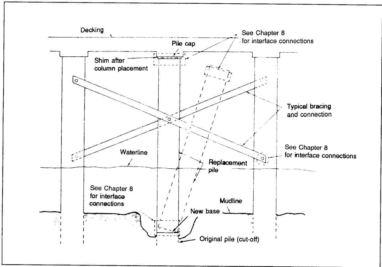
Figure A-6. Wood Columns
