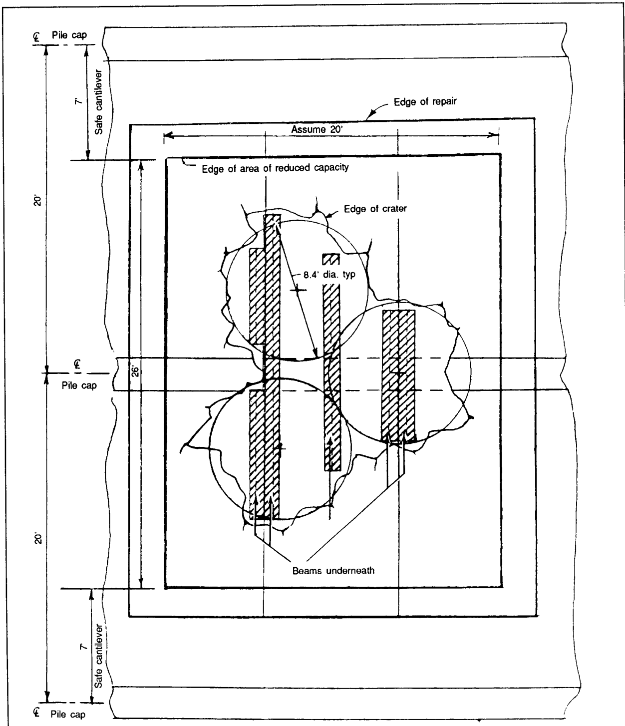
Figure A-35. Steel Plate Reinforced with Steel Beams (Repair for Case 3 Damage - 60 Foot of Steel Beam Required, Three 1-inch Thick, 8- by 30-foot Plates Required - Reinforced Plate Subconcept)
