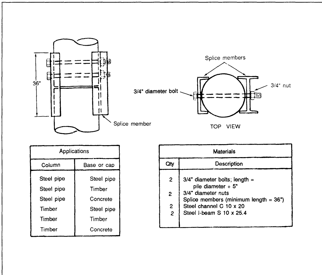
Figure A-23. Joining Like-Diameter Piles, Column to Base or Cap Connections (Connecting Method 2)
