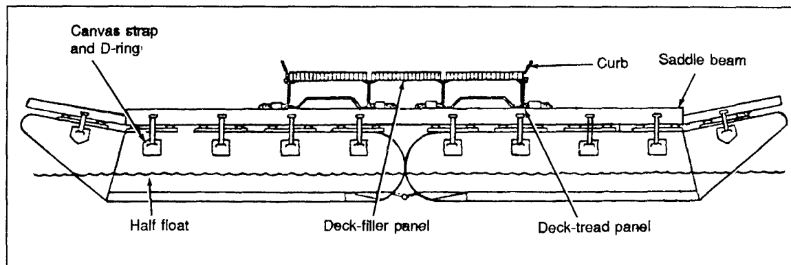
Figure 10-2. Causeway
