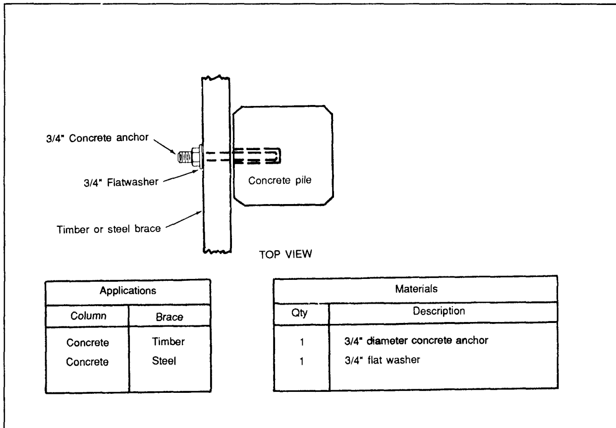
Figure A-21. Brace Connected to Concrete Pile with Concrete Anchor (Bracing Method 4)
