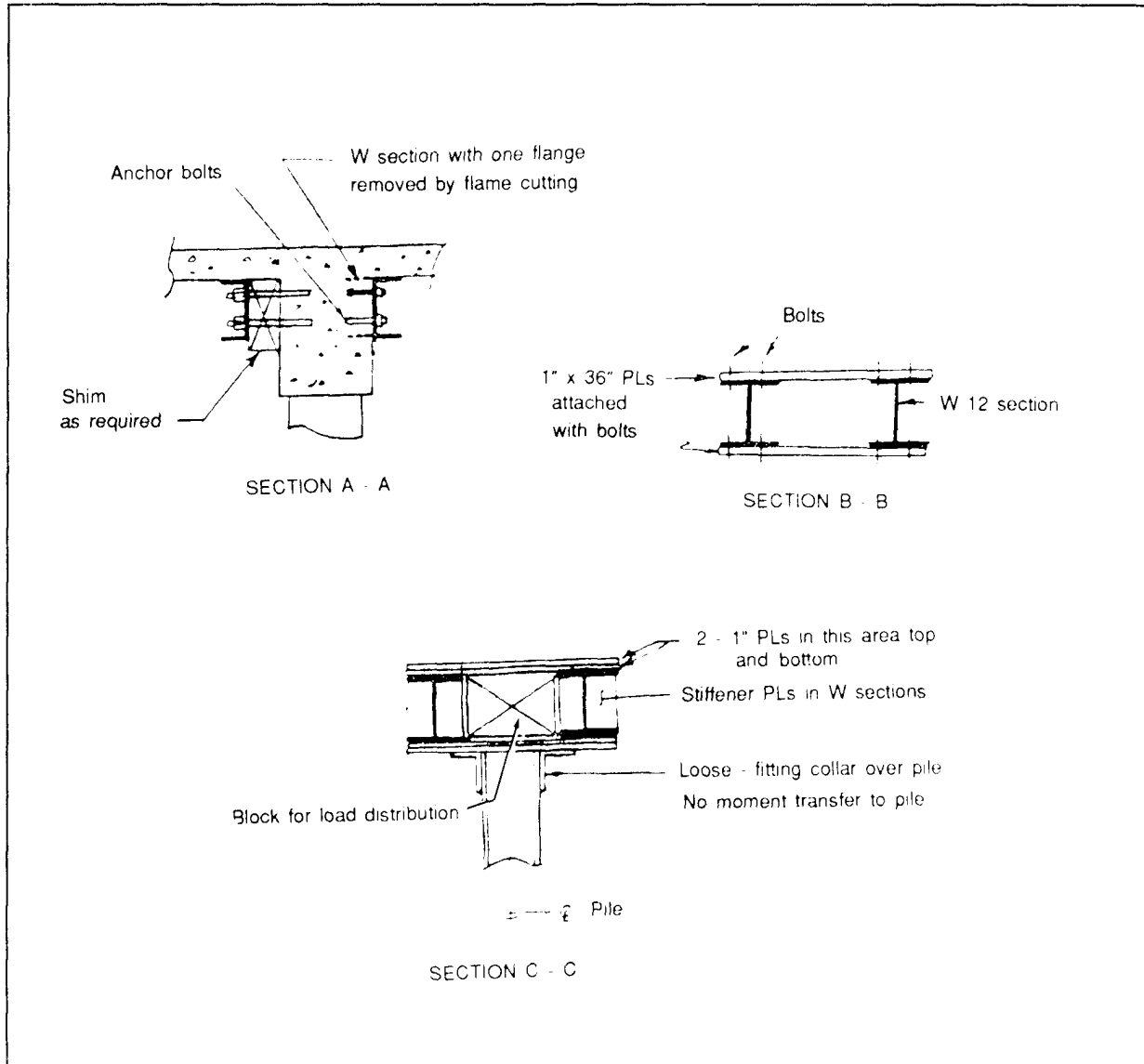
Figure A-37. Cross Sections of an Expedient Pile Cap
