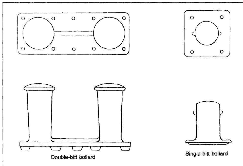
Figure 9-1. Single- and Double-Bitt Bollards
