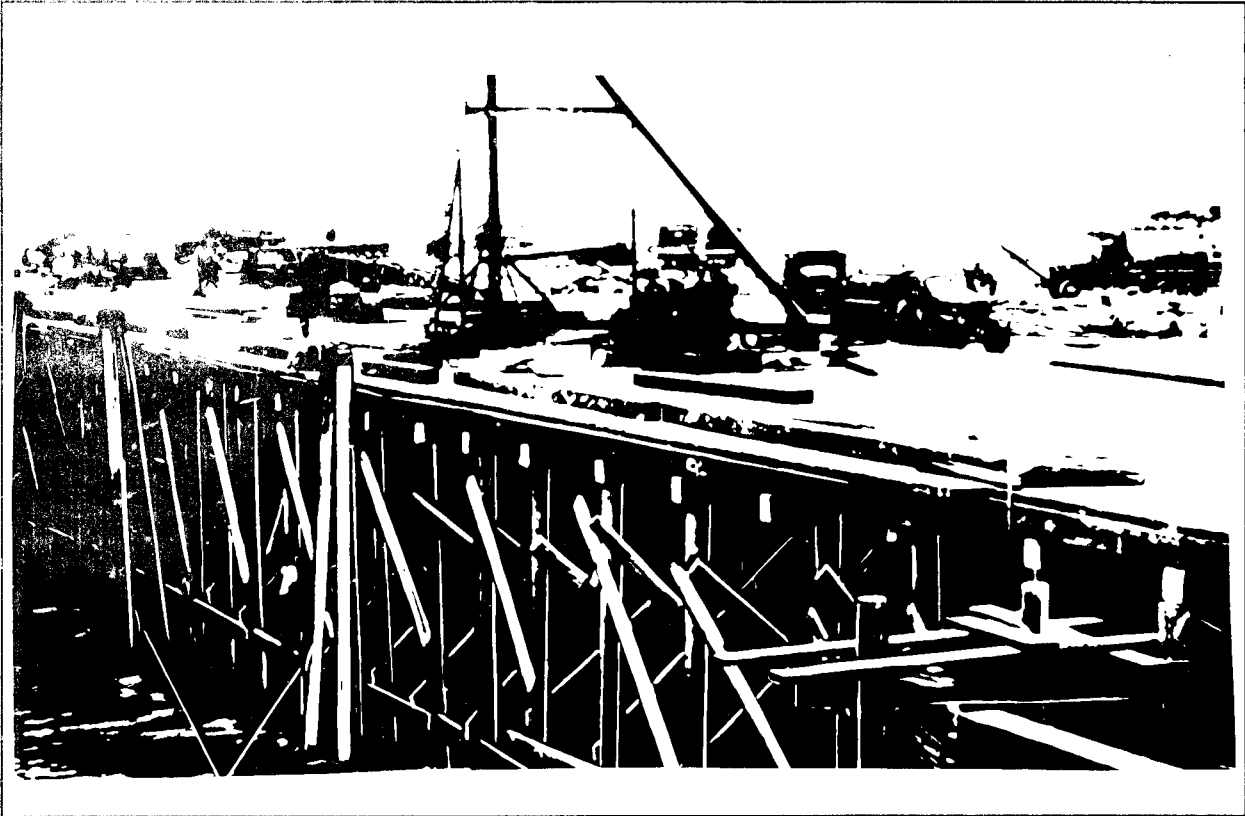
Figure 8-11. Transverse, Longitudinal, and Horizontal Bracing for Extreme Tidal Range
