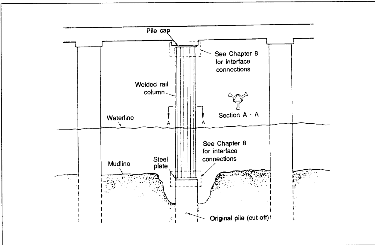
Figure A-9. Welded Steel Rail Column
