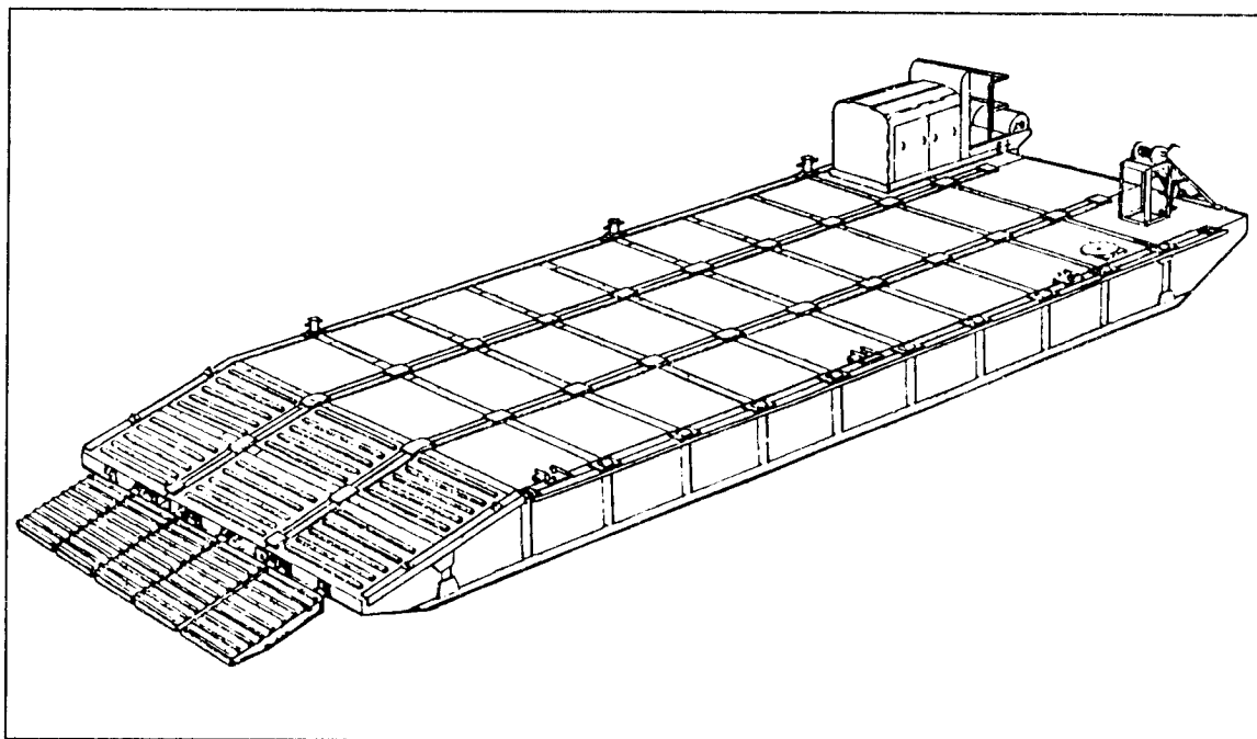
Figure 10-9. Sloping Barge with Ramp Attached
