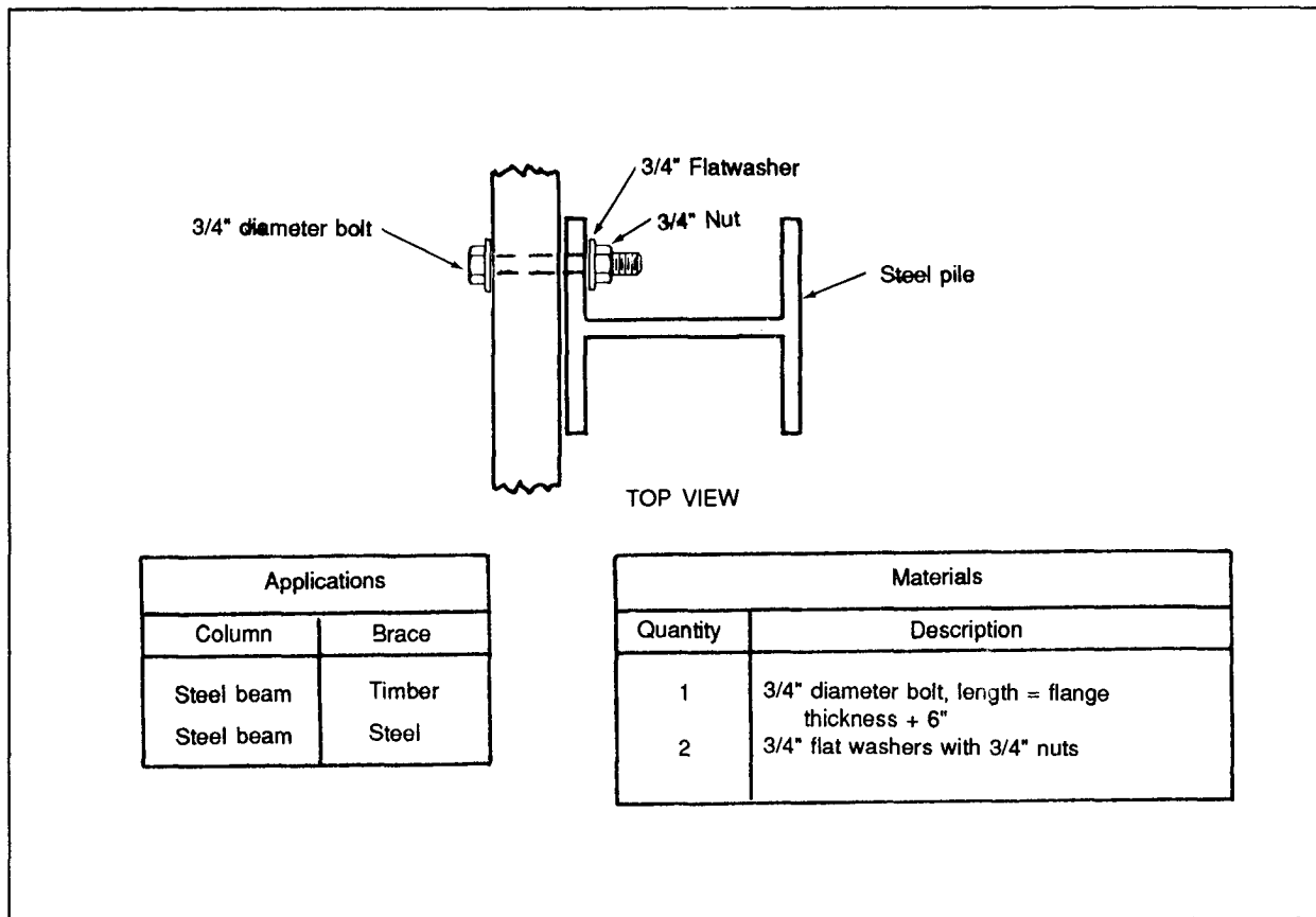
Figure A-19. Brace Connected to Steel Beam Pile (Bracing Method 2)
