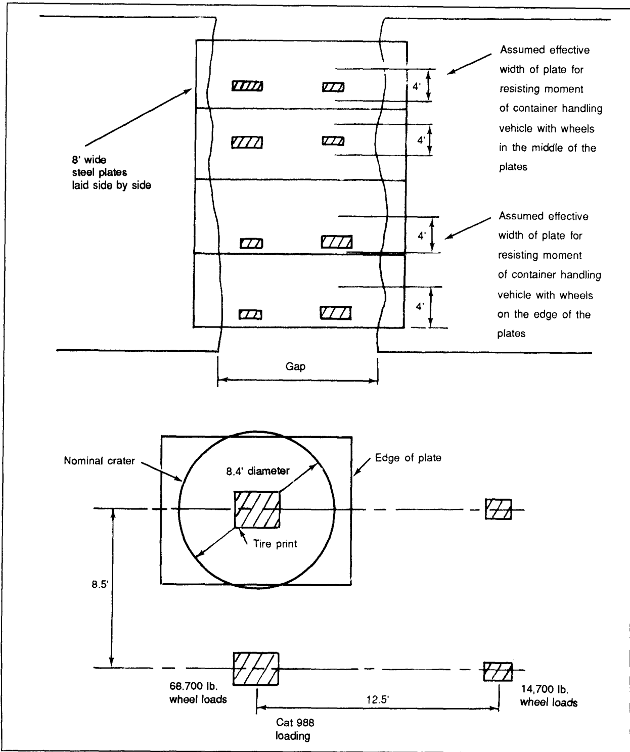
Figure A-29. Assumptions for Plate Repair Design
